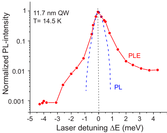
FIG. 7. (Color online) PLE and PL spectra of the 11.7 nm QW at T=14.5 K.
