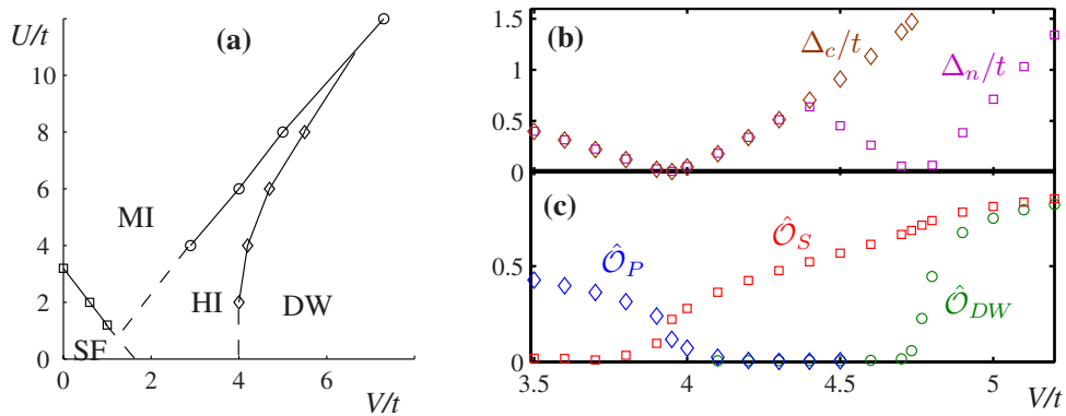
FIG. 4. (Color online) (a) Phase diagram of a single unperturbed chain in the space of (U/t, V/t) , obtained from the numerical calculations. (b) The charge ( \diamond ) and neutral ( \square ) gaps along the same cut through the three insulating phases. The charge gap vanishes at the MI-HI transition, whereas only the neutral gap vanishes at the transition to the DW phase. (c) The parity ( \diamond ), string ( \square ) and Density wave ( \circ ) order parameters as a function of V/t along a line of constant U/t=6 . The string and parity orders are defined as the square roots of Eqs. (12) and (13), respectively.
