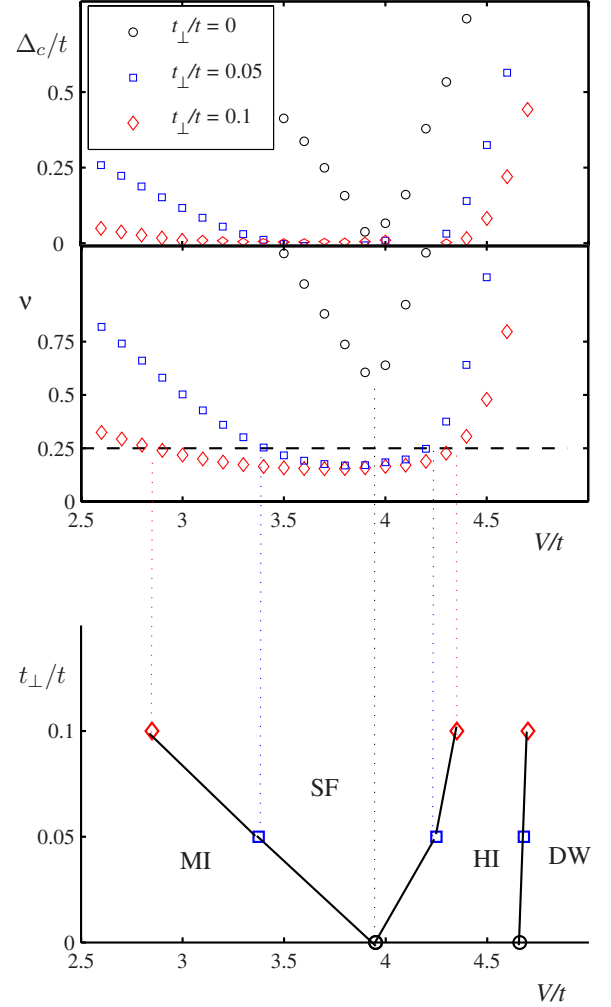
FIG. 8. (Color online) Effect of interchain tunnel coupling on the phase diagram. (a) Calculated charge gap as a function of V/t at constant U/t=6 for different values of the interchain tunneling t_{\perp} . The gaps were obtained by extrapolation to an infinite chain through finite-size scaling analysis. The fact that the estimate for the gap are sometimes slightly negative is due to errors in the extrapolation. Note the gapless phase that appears between the two insulating phases. (b) Power-law fit for the spatial decay of the single-particle density matrix for the same cuts through the phase diagram. The fact that \nu < 1/4 in the gapless phase confirms that it is indeed a superfluid. The transition to the gapped phase seems to occur at the universal exponent \nu=1/4 consistent with a Kosterlitz-Thouless transition. (c) Evolution of the phase boundaries with t_{\perp} inferred from the calculations.
