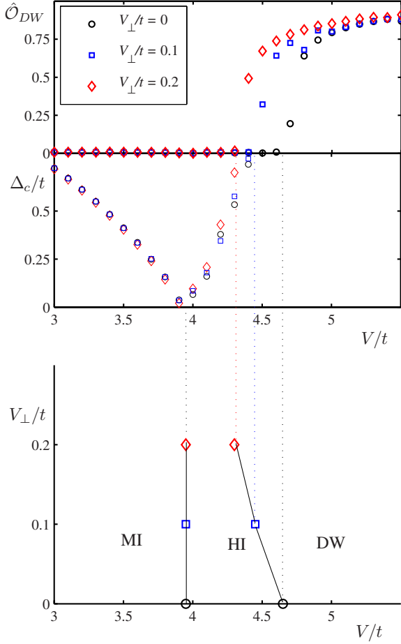
FIG. 7. (Color online) Effect of interchain interaction coupling on the phase diagram. (a) Calculated DW order parameter as a function of V/t at constant U/t=6 for different values of the interchain interaction V_{\perp} . (b) Calculated charge gap on the same cut through the phase diagram and the same values of V_{\perp} . (c) Evolution of the phase boundaries with V_{\perp} inferred from the calculations.
