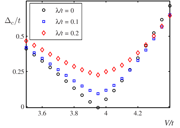
FIG. 6. (Color online) Charge gap as a function of V/t at constant U/t=6 for different values of the inversion-symmetry-breaking perturbation. \lambda is defined in Eq. (26).
