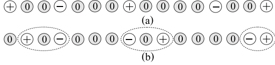
FIG. 2. Typical configurations in the (a) HI and (b) MI ground states. The numbers represent \delta n (the deviation of the local occupation from the average density). The HI can be described as a charge ordered +, -, +, \dots state with an undetermined number of 0 sites between each + and - . The MI is a dilute gas of particle-hole pairs (indicated by the dotted line).
