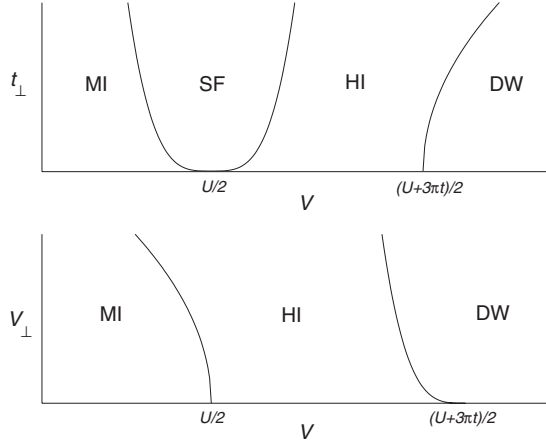
FIG. 3. Evolution of the phase diagram with interchain coupling predicted from bosonization. (a) Plane of the nearest-neighbor interaction V versus t_{\perp} (interchain tunneling) at fixed on-site interaction U and no interchain repulsion. (b) In the plane of V versus V_{\perp} (interchain repulsion) at t_{\perp}=0 and fixed U .
