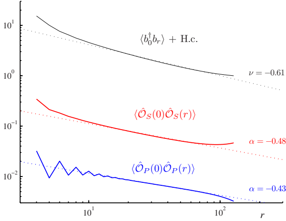
FIG. 5. (Color online) Decay of the parity and string correlations and of the single-particle density matrix at the HI-MI transition. The power-law fits are consistent with the field theoretical predictions for the relations between the different decay exponents (see text).
