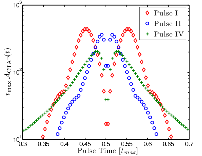
FIG. 8. (Color online) \mathcal{A}_{\text{CTAP}}(t) plotted for three different pulse sequences (pulse III is not included as it requires excessively long pulse times). From this plot we can estimate that for the chosen values of V_{\text{max}} and V_{\text{min}} , the pulse time must be at least t_{\text{max}} \geq 1/100(E^*)^{-1} to ensure adiabatic evolution.
