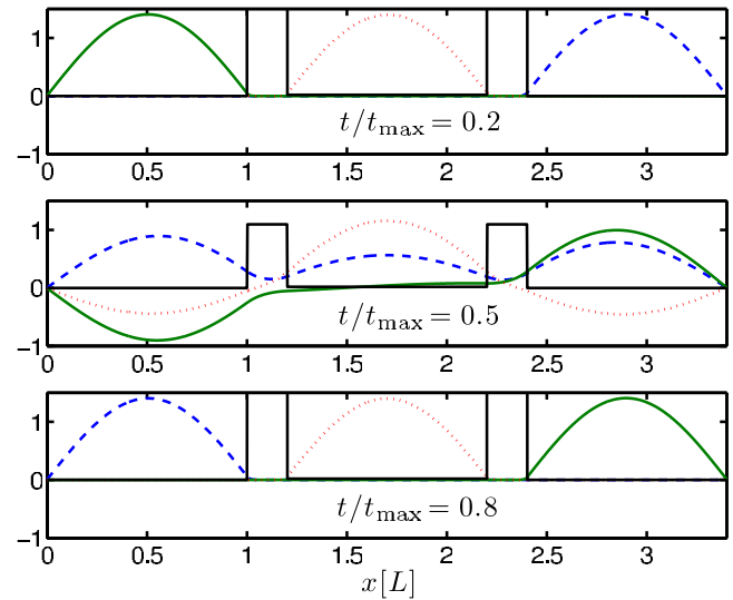
FIG. 6. (Color online) Eigenstates of the three well system as a function of time within pulse I plotted at (a) t/t_{\max}=0.2 , (b) t/t_{\max}=0.5 , and (c) t/t_{\max}=0.8 . The eigenstates are the ground state (dashed), first excited (solid) and second excited state (dotted), respectively, where the CTAP pulse corresponds to the first excited state. Note, the potential is shown in arbitrary units for comparison.
