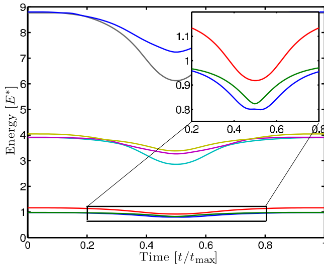
FIG. 5. (Color online) Eigenspectrum of the three well system as a function of time within pulse sequence II. The insert shows the three lowest eigenvalues in the central region of interest where the characteristics of the eigenstates are changing fastest.
