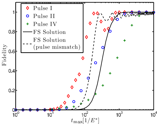
FIG. 12. (Color online) Fidelity of the pulse as a function of the total pulse time, shown for three different pulses. The FS solution to this problem is also shown (solid line) with Gaussian overlapping pulses as well as the same problem with a timing mismatch (dashed line) such that the time separation between the pulses is doubled. The oscillations in the fidelity stem from this imperfect overlap in the pulses.
