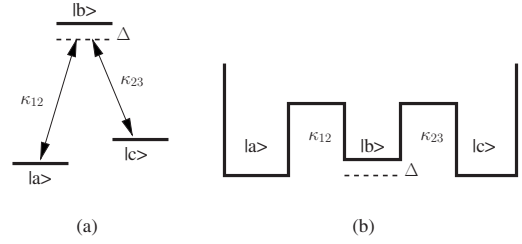
FIG. 3. Correspondence of the (a) quantum optics description of a three level atom with laser transitions which is equivalent to the finite state approximation and (b) a single electron undergoing coherent tunneling between one of three finite wells (SW). The tunnel matrix elements between states are \kappa_{12} and \kappa_{23} , while the single-photon detuning (central well offset energy) is given by \Delta .
