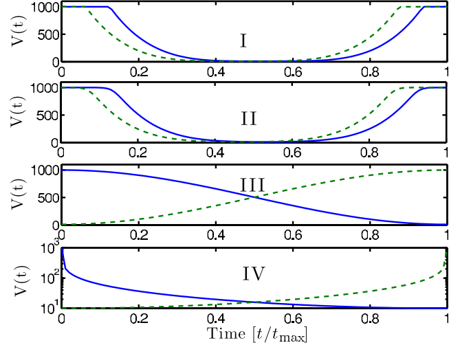
FIG. 4. (Color online) Four different pulsing schemes for modulation of a barrier height to result in a CTAP transfer between wells. In each case, the solid (dashed) curve is the height of barrier 1 (2) as a function of pulse time. Note the logarithmic scale for pulse IV.
