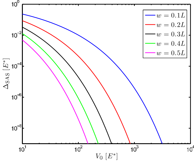
FIG. 2. (Color online) The energy gap between the ground and excited states ( \Delta_{\text{SAS}} ) as a function of the barrier height V_0 in units of E^* , for a double-well system comprised of wells of width L separated by a barrier of width w , as shown in Fig. 1.
