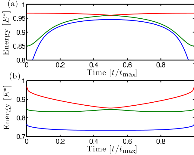
FIG. 7. (Color online) Eigenspectrum of the three well system as a function of time for (a) pulse III and (b) pulse IV. Note the very small energy gap for pulse III, due to the smaller tunneling rate at the midpoint of the pulse sequence.
