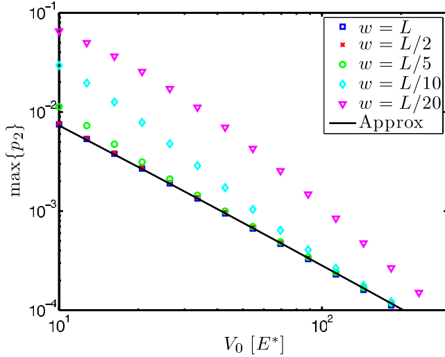
FIG. 9. (Color online) Occupation probability of the central region as a function of barrier height and barrier width. Note that for sufficiently high barriers, the occupancy is largely independent of barrier width. Even with the barrier at its minimum value during a CTAP pulse, the population of the central well and the barriers is less than 0.1 for a barrier width of w=L/20 .
