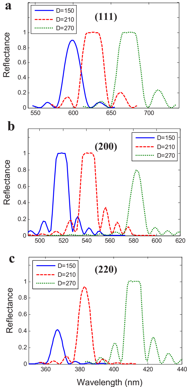
FIG. 9. (Color online) Wavelength (in vacuum) dependence of the integrated intensity of light specularly diffracted by 25 (111) CCA layers each containing 500 \times 500 particles. The incident light is normal to the (a) (111), (b) (200), and (c) (220) planes. The CCA consist of spheres with diameters of 150 nm (blue), 210 nm (red), and 270 nm (green).
