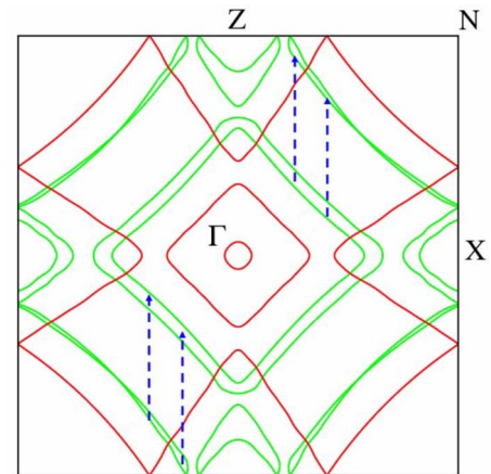
FIG. 5. (Color online) Fermi surface at k_y=0 . Red and green lines approximately indicate sections of FS formed by 5p orbitals from the single and double Te layers, respectively. Arrows indicate the on-axis lattice modulation wave vector expressed in the reduced BZ, \vec{q}' = c^* - \vec{q} \sim (1/3)c^* observed in SADP for \text{Nd}_2\text{Te}_5 , \text{Sm}_2\text{Te}_5 , and \text{Gd}_2\text{Te}_5 .
