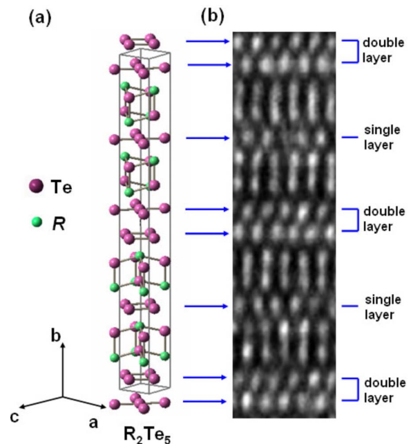
FIG. 1. (Color online) (a) Schematic diagram showing the average (unmodulated) crystal structure of R_2Te_5 . b axis is vertical in the figure. Solid gray lines indicate a unit cell. (b) High resolution TEM of Gd_2Te_5 along the [101] direction showing alternating single and double Te layers.
