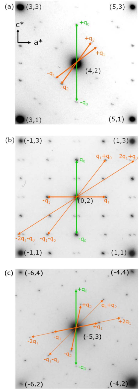
FIG. 3. (Color online) SADPs along the (010) zone axis at room temperature for (a) \text{Nd}_2\text{Te}_5 , (b) \text{Sm}_2\text{Te}_5 , and (c) \text{Gd}_2\text{Te}_5 . Bragg peaks are labeled by (hl) . Systematic modulation wave vectors are listed in Table II.
