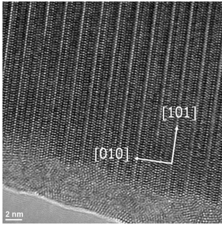
FIG. 2. High resolution TEM image of \text{Gd}_2\text{Te}_5 at room temperature as viewed looking down the [\bar{1}01] direction. The image shows a regular crystal structure over a macroscopic length scale (more than 25 nm) without intercalation or stacking faults in the layering along the b direction.
