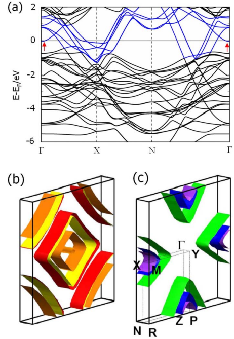
FIG. 4. (Color online) (a) Band structure of R_2\text{Te}_5 calculated by LMTO for R=\text{Lu} . The blue solid lines arise from Te 5p states in the square planar layers. [(b) and (c)] The resulting Fermi surfaces, illustrating the trilinear splitting that arises due to coupling between the three Te planes. Red and yellow sheets in (b) and blue and purple sheets in (c) indicate the weaker bilayer splitting originating from a Te double layer, while orange and green sheets in (b) and (c) are due to a Te single layer and the splitting is significant. The \Gamma point at the center of the zone and other high symmetry points have been labeled.
