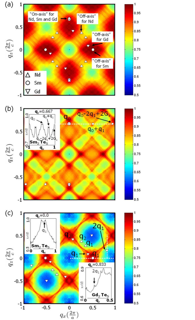
FIG. 6. (Color online) Color scale for all panels: red high, blue low. (a) The Lindhard susceptibility, \chi(\vec{q}) = \sum_{nn'} \chi_{nn'}(\vec{q}) at q_y=0 , summed for all the bands including inter single-double layer pairs. (b) \chi_D(\vec{q}) : contribution to \chi(\vec{q}) from the double Te layers. On-axis wave vectors for all three compounds lie on the global maximum. Inset: A line cut following the dashed line, illustrating the resonant enhancement of the mixed harmonics \vec{q}_0 + \vec{q}_1 and \vec{q}_0 - 2\vec{q}_1 + 2\vec{G}_x for \text{Sm}_2\text{Te}_5 . (c) \chi_S(\vec{q}) : contribution to \chi(\vec{q}) from the single Te layers. Symbols represent first harmonics of the off-axis modulation vectors for all three compounds and second harmonics for \text{Gd}_2\text{Te}_5 . Upper inset: A line cut following the horizontal dashed line. The off-axis modulation lies close to the global maximum of \chi_S(\vec{q}) for \text{Sm}_2\text{Te}_5 . Lower inset: A line cut following the vertical dashed line, showing the resonant enhancement of the commensurate off-axis lattice modulation for \text{Gd}_2\text{Te}_5 .
