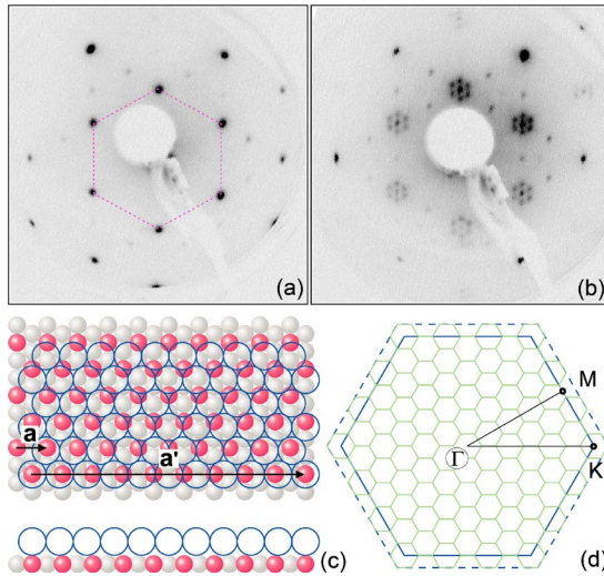
FIG. 1. (Color online) LEED pattern of the Ag(111) (\sqrt{3} \times \sqrt{3})R30^\circ -Bi surface alloy (a) before and (b) after Xe adsorption. The reciprocal space hexagonal unit cell of the alloy is traced in (a) for clarity. (c) Schematics (top and side views) of a commensurate 9 \times 9 Xe-Ag(111) (\sqrt{3} \times \sqrt{3})R30^\circ -Bi structure, showing the hexagonal unit vectors \mathbf{a} of the substrate and \mathbf{a}' = 9\mathbf{a} of the superlattice. Ag, gray filled circles; Bi, red (dark gray) filled circles; Xe, empty circles. The relaxations of the BiAg 2 layer and of the overlayer are neglected. (d) The surface BZs of the substrate are shown in blue (black) and that of the superlattice in green (gray). The large dashed hexagon is the BZ of the isolated Xe overlayer.
