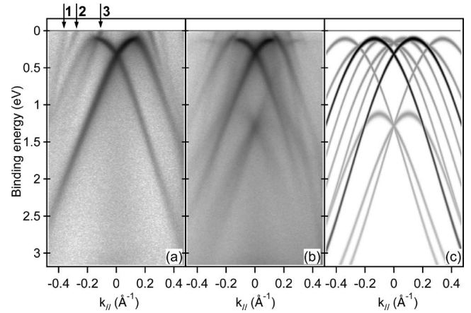
FIG. 2. The measured band structure along the \bar{M}\bar{\Gamma}\bar{M} high-symmetry direction (a) before and (b) after Xe adsorption. k_{||}=0 corresponds to the \bar{\Gamma} point. The intensity is plotted on a logarithmic scale to enhance the weaker backfolded features. (c) shows a simple calculation of the expected band dispersion for an umklapp of the two high intensity bands in panel (a) according to a 9 \times 9 superperiodicity. Only the six BZs surrounding the central one are taken into account.
