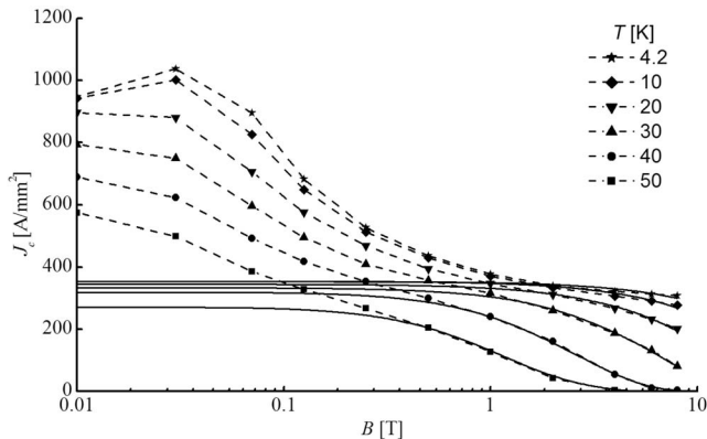
FIG. 17. Transport J_c of Bi-2223 tape B-2 measured as a function of magnetic field applied perpendicular to the tape surface. The solid lines represent the critical current density of the strongly linked backbone according to classical flux-creep theory [Eq. (12)]. The dashed lines are a guide to the eye.
