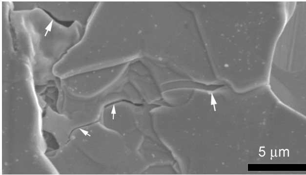
FIG. 9. SEM image of the grain structure of Bi-2223 tape B-4 showing cracks (arrows) after tensile strain exceeding \varepsilon_{\text{irr}} is applied in situ . The exact amount of applied strain is unknown, due to the partial etching of the tape surface.
