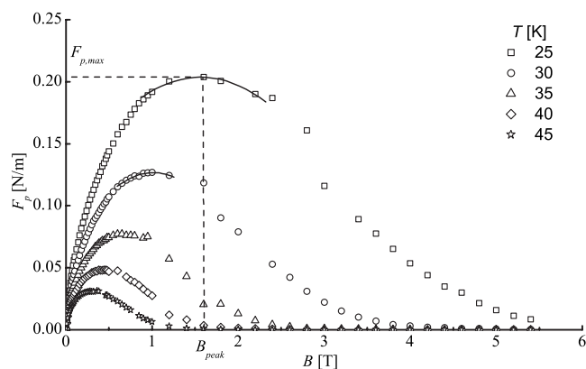
FIG. 3. Macroscopic pinning force as a function of magnetic field at various temperatures of tape B-2. The magnetic field is applied perpendicular to the tape surface. The solid lines are a second-order polynomial fit around the maximum of the pinning force.
