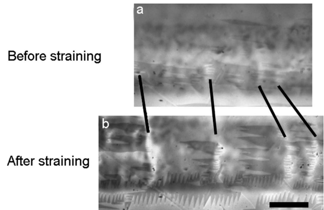
FIG. 8. (a) MO image of part of a Bi-2223 filament (oriented horizontally) in tape B-3 before axial strain is applied. The filament is partly shielded from the external magnetic field of 25 mT (dark areas). (b) Less dense areas form filament-wide cracks after strain is applied (bright areas), starting at a strain of \sim 0.6\% . The scale bar represents 125 \mu\text{m} .
