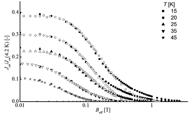
FIG. 14. Normalized critical current density of the weakly linked network as a function of effective magnetic field component ( B_{\text{eff}} ) at different temperatures for magnetic fields applied parallel (open symbols, B_{\text{eff}} = B/b_{scw} ) and perpendicular (solid symbols, B_{\text{eff}} = B ) to the surface of tape 2. Open and solid symbols of the same type correspond to the same temperature.
