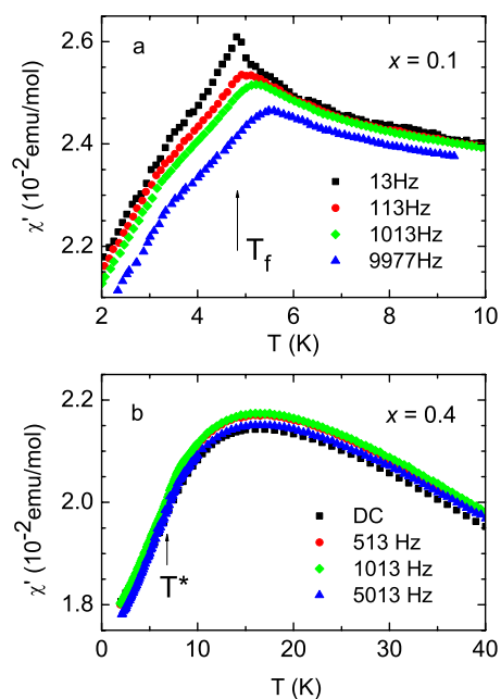
FIG. 4. (Color online) Temperature dependences of the real part of the ac susceptibility for different frequencies for the samples: (a) x = 0.1 and (b) x = 0.4 . The static (dc) susceptibility is also shown. The arrows mark the freezing temperature T_f and the temperature of the inflexion point of the susceptibility T^* .
