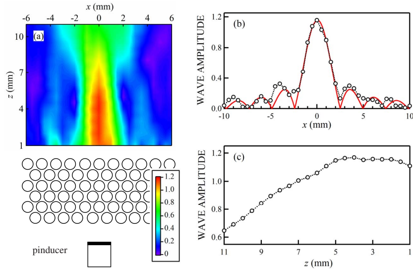
FIG. 6. (Color online) The experiment on imaging the field of the pinducer at 0.70 MHz with a flat phononic crystal filled with and immersed in water. (a) 2D image plot of the wave field amplitude. The color scale shows the normalized amplitude as described in the text. (b) Field profile obtained from the image plot by plotting the amplitude along the x direction at z=2.9 mm (open circles connected with a dashed line) and fit of the absolute value of the sinc function (red solid line). (c) Field profile obtained from the image plot by plotting the amplitude along the z direction at x=0 mm.
