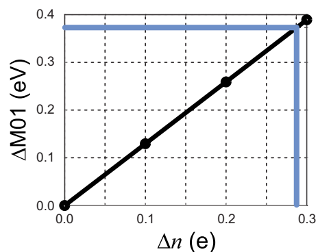
FIG. 8. (Color online) Shift of the lowest-lying molecular orbital (MO1) energy for geometry 2 , \Delta\text{MO1} , as a function of extra partial electronic charge, \Delta n . The thick horizontal line indicates the energy difference of the MO1 between the whole structure and geometry 2 .
