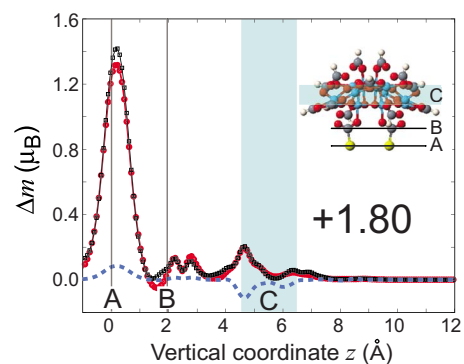
FIG. 9. (Color online) Filled circles : Spin magnetic moment difference between the whole structure and geometry 2 . The difference of the total magnetic moment is 1.80\mu_B when the spin density difference is integrated from z=-0.93 to z=12 Å. Empty squares : Magnetic moment difference between geometry 3 and 2 . Dashed curve : Magnetic moment difference between geometries 4 and 2 . The inset shows lines A and B and region C .
