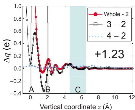
FIG. 7. (Color online) Filled circles : Charge density difference between the whole structure and geometry 2 vs the z coordinate. A , B , and C denote the locations of the S atoms (at z=0.09 Å), the bonding C atoms, and the Mn ions illustrated in the inset of Fig. 9. Upon integration from z=0.09 ( z=-0.93 ) to z=12.00 Å, a total of 1.23 (23.15) electrons is transferred from the surface to the molecule. Empty squares : Charge density difference between geometries 3 and 2 . Dashed curve : Charge density difference between a molecule with extra 0.3 electrons added to geometry 2 (denoted geometry 4 ) and a neutral molecule with geometry 2 .
