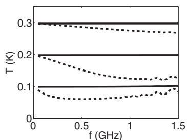
FIG. 3. Equilibrium temperature as a function of pump frequency for three different phonon bath temperatures. The temperature of resistor 1 (volume, 10^{-21} \text{ m}^3 ) is shown with a dashed line, while the temperature of resistor 2 (volume, 10^{-18} \text{ m}^3 ) is shown with a solid line. The bath temperatures T_{ph} \approx T_2 from top to bottom are 0.3 \times \hbar\omega_2/k_B , 0.2 \times \hbar\omega_2/k_B , and 0.1 \times \hbar\omega_2/k_B . Otherwise, the parameters are like in Fig. 2.
