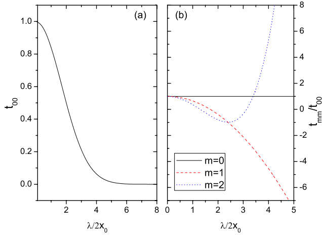
FIG. 1. (Color online) (a) The overlap t_{00} and (b) t_{mm} ( m = 0, 1, 2 ) scaled by t_{00} , as functions of the distance \lambda/2 between two neighboring centers in unit of the Gaussian half-width x_0 . We use t_{mn}(a) = \int_{-\infty}^{\infty} \varphi_m^*(x) \varphi_n(x-a) dx , where \varphi_n(x-a) denotes the eigenstate of the n th energy level of the harmonic oscillator with center at x = a .
