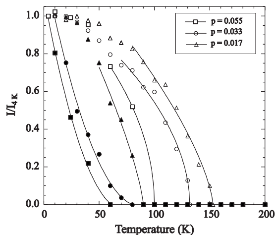
FIG. 11. Temperature variations of the integrated \frac{1}{2}\frac{1}{2}2 (bold symbols) and composite \frac{1}{2}\frac{1}{2}0 + (\frac{1}{2}\frac{1}{2}1) (open symbols) magnetic diffraction peak intensities (relative to 4 K values) for \text{RuSr}_2\text{Nd}_{0.9}\text{Y}_{0.2}\text{Ce}_{0.9}\text{Cu}_2\text{O}_{9.967} ( p=0.017 ), \text{RuSr}_2\text{Nd}_{0.9}\text{Y}_{0.2}\text{Ce}_{0.9}\text{Cu}_2\text{O}_{9.983} ( p=0.033 ), and \text{RuSr}_2\text{Nd}_{1.0}\text{Y}_{0.2}\text{Ce}_{0.8}\text{Cu}_2\text{O}_{9.955} ( p=0.055 ) showing the Ru and Cu spin ordering transitions. Critical law fits in the range T_c/2 < T < T_c are shown except for the p=0.033 and p=0.055 , and I(\frac{1}{2}\frac{1}{2}2) data which are fitted by an arbitrary curve.
