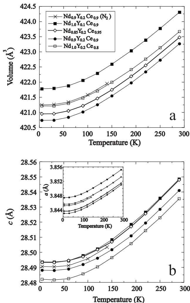
FIG. 9. Temperature variations of (a) unit-cell volume and (b) lattice parameters c and a (inset) for representative \text{RuSr}_2(\text{Nd}, \text{Y}, \text{Ce})_2\text{Cu}_2\text{O}_{10-\delta} samples.
