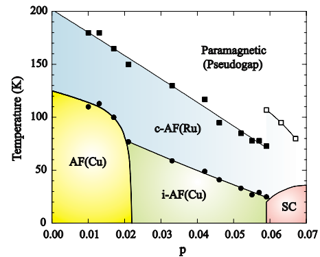
FIG. 3. (Color online) Electronic phase diagram for 1222-type ruthenocuprates. Ordering temperatures for the Ru spins ( T_{\text{Ru}} , squares) and Cu spins ( T_{\text{Cu}} , circles) at hole dopings p < 0.06 are from \text{RuSr}_2\text{Nd}_{1.8-x}\text{Y}_{0.2}\text{Ce}_x\text{Cu}_2\text{O}_{10-\delta} phases and \text{RuSr}_2\text{NdY}_{0.1}\text{Ce}_{0.9}\text{Cu}_2\text{O}_{9.967} in this study. T_{\text{Ru}} (open squares) and superconducting critical temperatures (diamonds) for \text{RuSr}_2\text{Gd}_{2-x}\text{Ce}_x\text{Cu}_2\text{O}_{10-\delta} ( x=0.6-0.8 ) samples are shown in the p=0.06-0.07 region.
