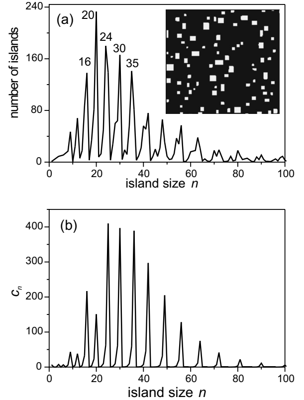
FIG. 4. Island size distribution of faceted islands obtained (a) in the kinetic Monte Carlo simulations and (b) by numerical solution of the Becker-Döring equations. The strong preference of magic island sizes is obvious.
