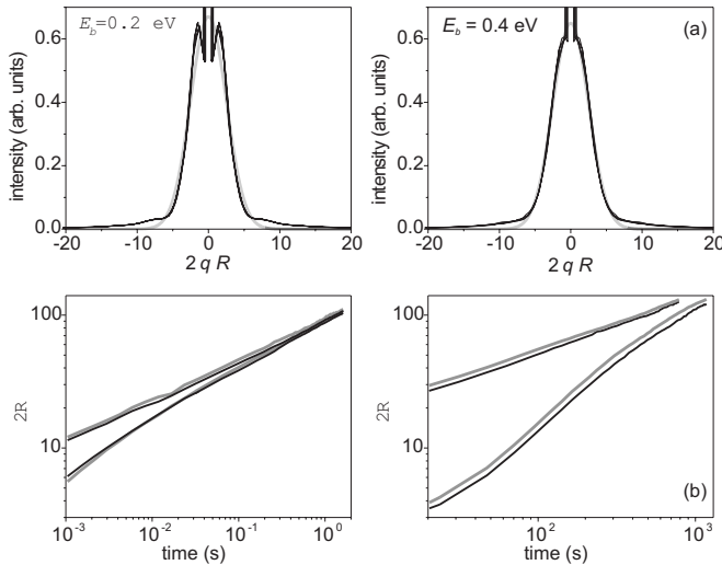
FIG. 2. (a) Diffraction peaks obtained from the Monte Carlo simulation results (the gray curves are Gaussian fits). (b) Time dependence of the average island sizes obtained from the numbers of atoms in the clusters (black curves) and from the widths of the diffraction peaks (gray curves).
