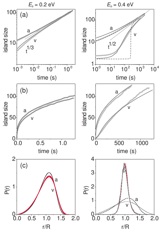
FIG. 5. (Color online) Results of numerical solutions of the Becker-Döring equations: time evolution of the average island sizes in (a) logarithmic and (b) linear scales and (c) the island size distributions. The left column presents calculations for a bond energy E_b=0.2 eV with diffusion-limited kinetics, while the right column shows the results for a bond energy E_b=0.4 eV with attachment-limited kinetics. The solutions of the Becker-Döring equations are shown in (a) and (b) by black lines, and the results of the kinetic Monte Carlo simulations by gray lines. Symbols “a” and “v” on the plots denote the results for adatom and advacancy islands, respectively. Full lines in the right column show the calculations for the discrete island energies with “magic” sizes, while the broken lines are calculations for the continuous Gibbs-Thomson chemical potential.
