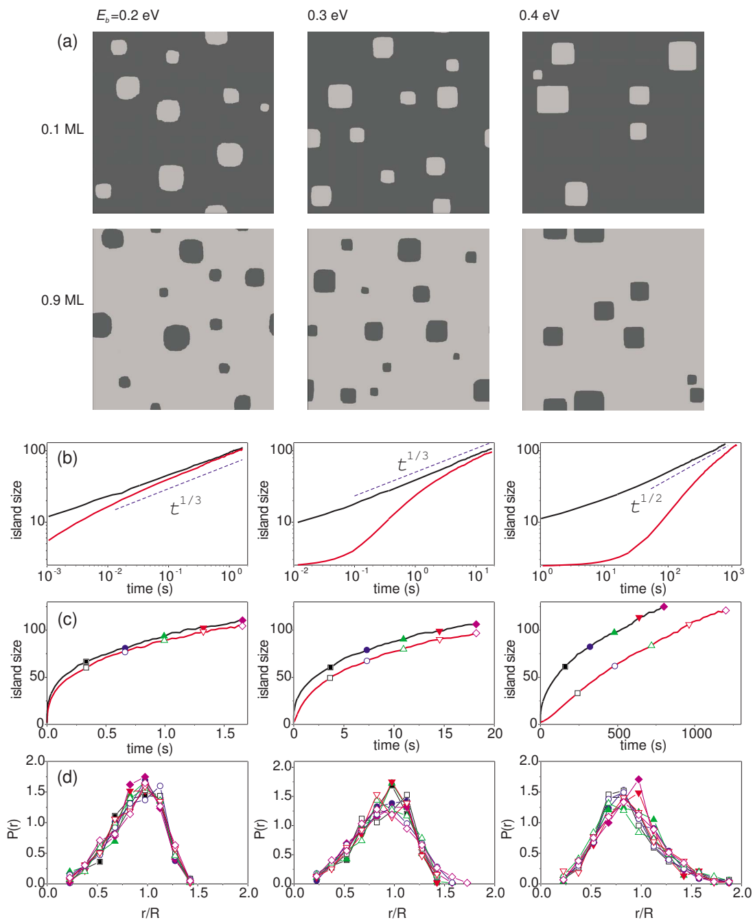
FIG. 1. (Color online) Results of kinetic Monte Carlo simulations: (a) snapshots of the 1000 \times 1000 simulation cells at the end of the simulations, (b) and (c) time dependence of the average island size in logarithmic and linear scales, and (d) the island size distributions. The gray levels in the snapshots vary from black to white as the surface height increases. Different columns show results for different bond energies E_b , with the temperature fixed at T=400 K. The size distributions are obtained at the time moments marked in (c) by the corresponding symbols.
