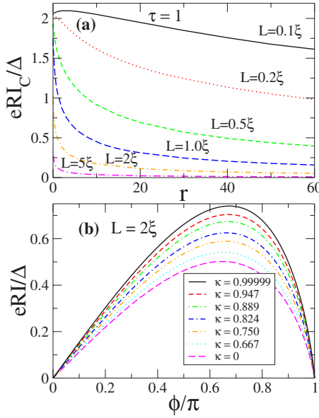
FIG. 7. (Color online) (a) Zero-temperature critical current of a diffusive SNS system with \tau=1 as a function of the parameter r=G_N/G_B for different lengths of the normal wire. (b) Current-phase relation at zero temperature for an asymmetric junction with L=2\xi and \tau=1 . The asymmetry parameter \kappa is defined as \kappa=1-r_R/r_L with r_R \leq r_L and r_L+r_R=r_{LR}=\text{const} . Here, r_{LR}=2 and r_L=1, 1.5, 1.7, 1.8, 1.9, 1.95, 1.99999 .
