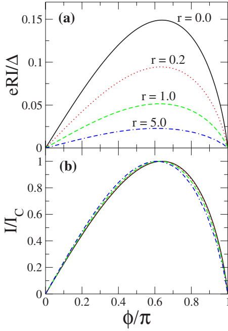
FIG. 5. (Color online) Zero-temperature supercurrent-phase relation of a diffusive SNS junction for L=8\xi ( \Delta=64\epsilon_T ) for different values of the ratio r=G_N/G_B and \tau=1.0 . In panel (a), we show the results for the product eRI/\Delta , where R is the normal-state resistance, while in panel (b), we have normalized the different curves by the critical current I_C .
