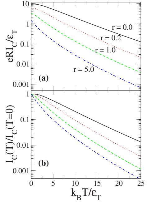
FIG. 6. (Color online) (a) Critical current of a diffusive SNS junction as a function of the temperature for L=8\xi and different values of the ratio r=G_N/G_B and \tau=1.0 . (b) The same as (a) but normalized by the critical current at zero temperature.
