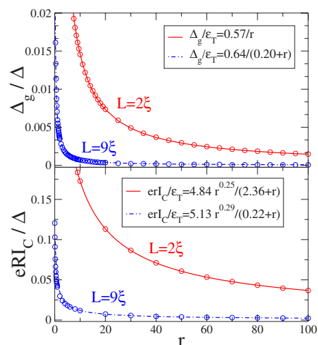
FIG. 12. (Color online) Minigap and critical supercurrent as a function of r for the two lengths L=2\xi and L=9\xi . The solid lines show the fitting curves of the numerically calculated data (circles) in units of the Thouless energy for r \gg 1 .
