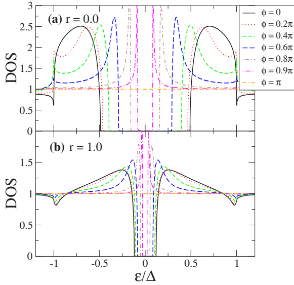
FIG. 3. (Color online) Density of states of a SNS junction as a function of energy in the middle of a wire of length L=2\xi ( \Gamma_{sf}=0 ) for different values of the superconducting phase difference \phi . The interfaces are identical and characterized by a ratio r=G_N/G_B=0.0 in panel (a) and r=1.0 in panel (b). In both cases, \tau=1 .
