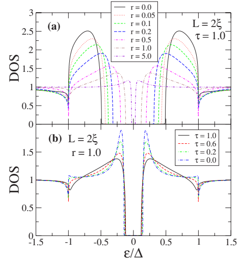
FIG. 1. (Color online) Density of states of a SNS junction as a function of energy in the middle of a wire of length L=2\xi without spin-flip scattering ( \Gamma_{sf}=0 ). The SN interfaces are assumed to be identical and there is no phase difference between the S electrodes. In panel (a), the different curves correspond to different values of the ratio r=G_N/G_B and a transmission \tau=1 , while in panel (b), they correspond to different values of the transmission \tau for a ratio r=1.0 .
