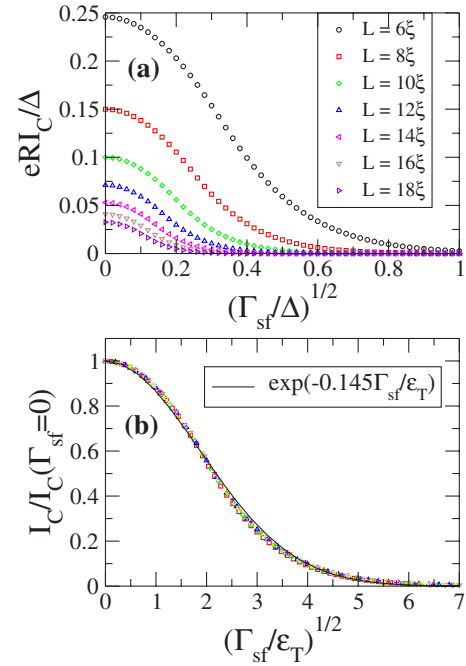
FIG. 8. (Color online) (a) Zero-temperature critical current of a diffusive SNS as a function of the spin-flip rate for different lengths of the normal wire and ideal interfaces ( r=0 ). (b) The same as (a) but the critical current is now normalized by the zero spin-flip rate value and \Gamma_{sf} is normalized by the Thouless energy of the wires. Notice that all the curves collapse into a single one that can be approximately described by the Gaussian function I_C/I_C(\Gamma_{sf}=0) = \exp(-0.145\Gamma_{sf}/\epsilon_T) shown as a black solid line.
