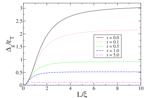
FIG. 2. (Color online) Minigap \Delta_g of a SNS junction as a function of the length of the N wire for different values of r=G_N/G_B and \Gamma_{sf}=0 . The contact is assumed to be symmetric and the transmission is set to \tau=1 . Notice that \Delta_g is normalized by the Thouless energy \epsilon_T .
