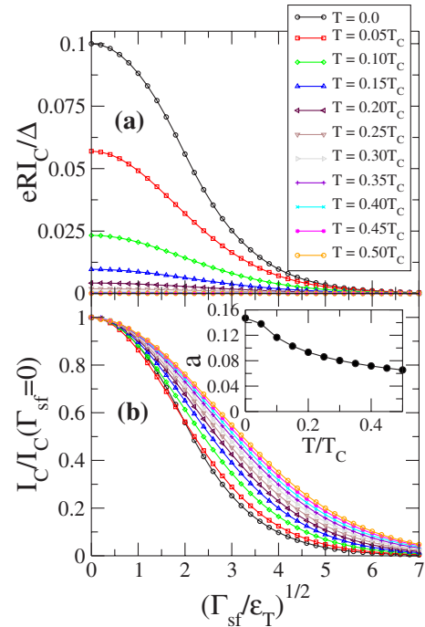
FIG. 10. (Color online) (a) Critical current for a wire length L=10\xi as a function of the spin-flip rate for different values of the temperature (in unit of the critical temperature T_C ). (b) The same as (a) but the critical current is normalized by its value at \Gamma_{sf}=0 . The inset shows the temperature dependence of the constant a used in the Gaussian fits: I_C/I_C(\Gamma_{sf}=0) = \exp(-a\Gamma_{sf}/\epsilon_T) .
