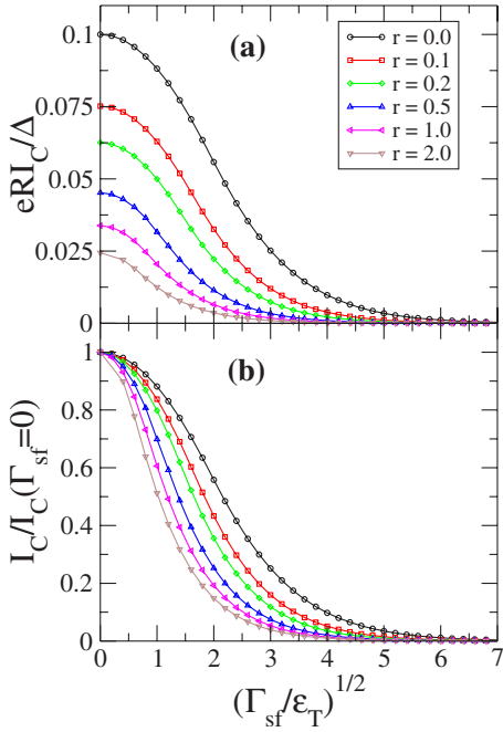
FIG. 9. (Color online) (a) Zero-temperature critical current for a wire length L=10\xi as a function of the spin-flip rate for different values of the interface resistance and \tau=0 . (b) The same as (a) but the critical current is normalized by its value at \Gamma_{sf}=0 .
