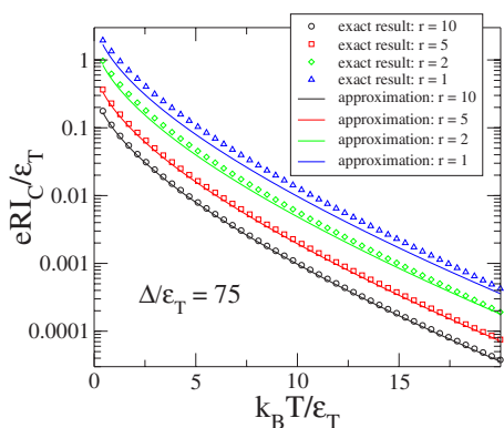
FIG. 11. (Color online) Comparison between the linearized result of Eq. (A9) and the exact numerical result for the temperature dependence of the critical current for a wire with \Delta=75\epsilon_T in the absence of spin-flip scattering ( \Gamma_{sf}=0 ). The different curves correspond to different values of the ratio r=G_N/G_B and in the exact result we have used \tau=0 .
