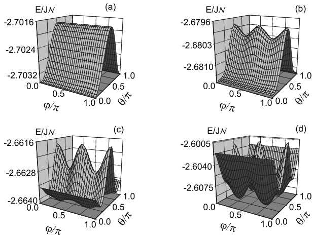
FIG. 2. Energy potentials of a spherical many-spin particle of \mathcal{N}=1736 spins on an sc lattice with uniaxial anisotropy in the core ( k_c=0.0025 ) and NSA with constant (a) k_s=0.005 , (b) k_s=0.112 , (c) k_s=0.2 , and (d) k_s=0.5 .
