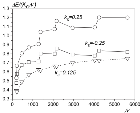
FIG. 17. Energy barriers vs \mathcal{N} for truncated octahedra with internal fcc structure and uniaxial core anisotropy with k_c=0.0025 .
