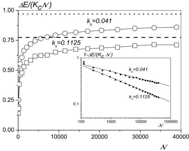
FIG. 16. Energy barrier as a function of the total number of spins \mathcal{N} for two different values of the surface anisotropy, spherical particles cut from the sc lattice with uniaxial anisotropy k_c=0.0025 in the core. The dotted and dashed lines correspond to analytical expressions in Eqs. (7) and (9). The inset shows a slow dependence of the difference between these results and the uniaxial one-particle energy barrier K_c\mathcal{N} in the logarithmic scale. The lines in the inset are the analytical expressions in Eqs. (7) and (9).
