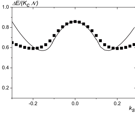
FIG. 13. Energy barrier as a function of k_s for a spherical particle cut from an sc lattice. The particle contains \mathcal{N}=20\,479 spins and has the uniaxial core anisotropy k_c=0.0025 . The solid line is a plot of the analytical expressions (1.1) and (2) from Table I, using Eqs. (7) and (9).
