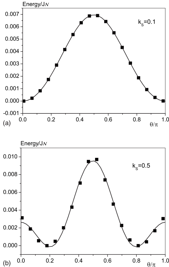
FIG. 3. (Shifted) 2D energy potentials of a spherical many-spin particle of \mathcal{N}=1736 spins on an sc lattice with uniaxial anisotropy in the core ( k_c=0.01 ) and NSA with constant (a) k_s=0.1 , (b) 0.5 . The solid lines are plots of Eq. (14).
