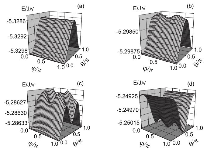
FIG. 8. Energy potentials of an ellipsoidal particle cut from an fcc lattice and with uniaxial anisotropy in the core ( k_c=0.0025 ) and NSA with constant (a) k_s=0.0125 , (b) k_s=0.075 , (c) k_s=0.1 , and (d) k_s=0.175 .
