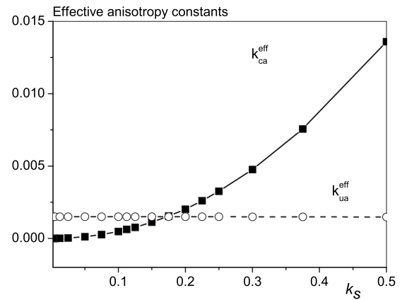
FIG. 7. Effective anisotropy constants against k_s for a spherical particle of \mathcal{N}=1264 spins cut from an fcc lattice with uniaxial core anisotropy k_c=0.0025 . The lines are guides for the eyes.
