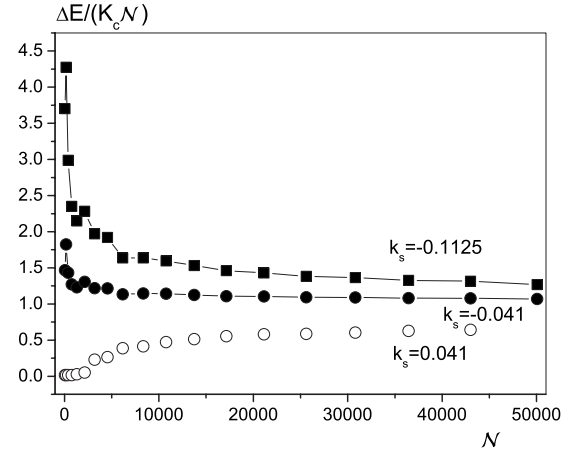
FIG. 18. Energy barriers as a function of the particle size for ellipsoidal particles with internal sc structure, uniaxial anisotropy k_c=0.0025 , and different values of k_s .
