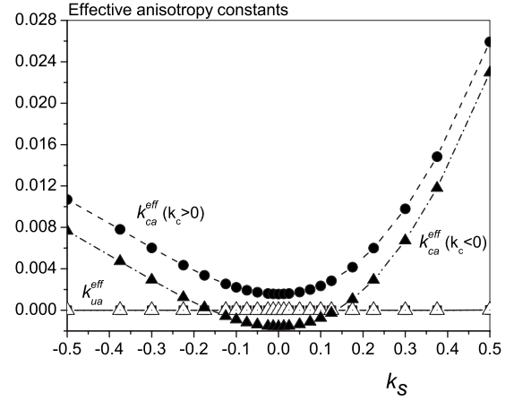
FIG. 10. Effective anisotropy constants against k_s for a regular truncated octahedral particle of \mathcal{N}=1289 spins, fcc structure, and cubic anisotropy in the core with k_c > 0 and k_c < 0 .
