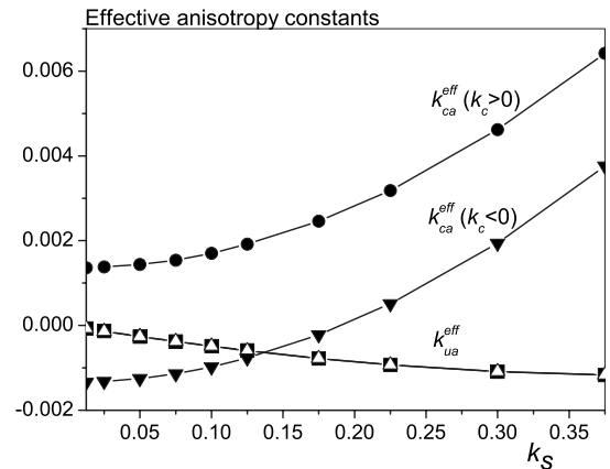
FIG. 11. Effective anisotropy constants against k_s for a truncated octahedral particle with different atomic densities on surfaces. The particle has \mathcal{N}=1080 spins, fcc structure, and cubic anisotropy in the core with k_c > 0 and k_c < 0 .
