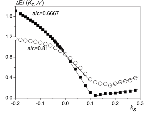
FIG. 15. Energy barriers vs k_s of ellipsoidal particles with different aspect ratio a/c=0.6667 , \mathcal{N}=21121 , and a/c=0.81 , \mathcal{N}=21171 , with uniaxial core anisotropy k_c=0.0025 . The solid lines are linear fits.
