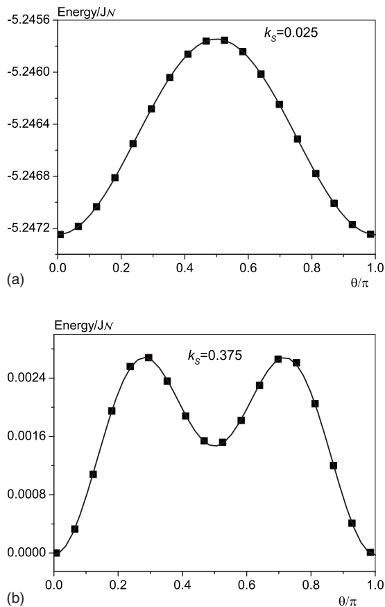
FIG. 6. The same as in Fig. 3 but here for the fcc lattice and k_s=0.025 and 0.375 .
