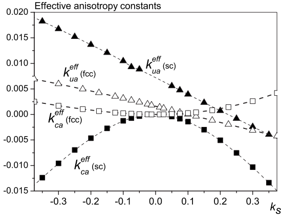
FIG. 9. Effective anisotropy constants against k_s for an ellipsoidal particle of \mathcal{N}=2044 spins on sc and fcc lattices, with uniaxial core anisotropy k_c=0.0025 . The lines are guides for the eyes.
