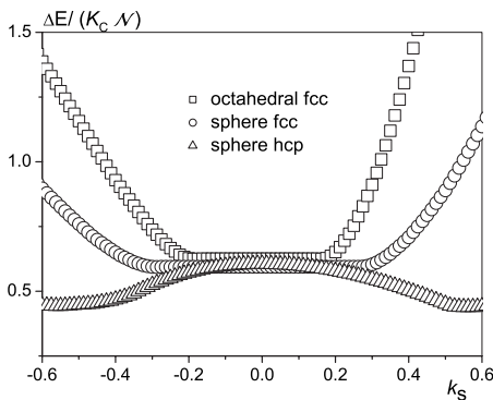
FIG. 14. Energy barriers against k_s for truncated octahedral particles cut from an fcc lattice ( \mathcal{N}=1688 ) and spherical particles cut from the fcc ( \mathcal{N}=1289 ) and hcp ( \mathcal{N}=1261 ) lattices. Uniaxial core anisotropy with k_c=0.0025 is assumed.
