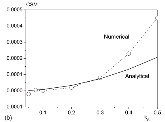
FIG. 4. Effective anisotropy constants against k_s for a spherical many-spin particle of \mathcal{N}=1736 spins cut from an sc lattice. (b) the CSM contribution obtained numerically as k_{ua}^{eff} , excluding the core uniaxial contribution from Eq. (7). The thick solid lines are plots of Eqs. (9) and (11) with \varphi=0 .
