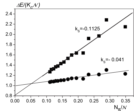
FIG. 19. Linear fit of energy barriers, vs the surface-to-total number of spins N_s/\mathcal{N} , of ellipsoidal particles with aspect ratio 2:3 with k_s=-0.041 (circles) and k_s=-0.1125 (squares).
