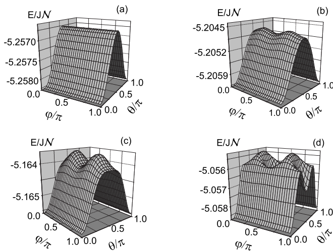
FIG. 5. Energy potentials of a spherical many-spin particle with uniaxial anisotropy in the core ( k_c=0.0025 ) and NSA with constant (a) k_s=0.005 , (b) k_s=0.1 , (c) k_s=0.175 , and (d) k_s=0.375 . The particle contains \mathcal{N}=1264 spins on an fcc lattice.
