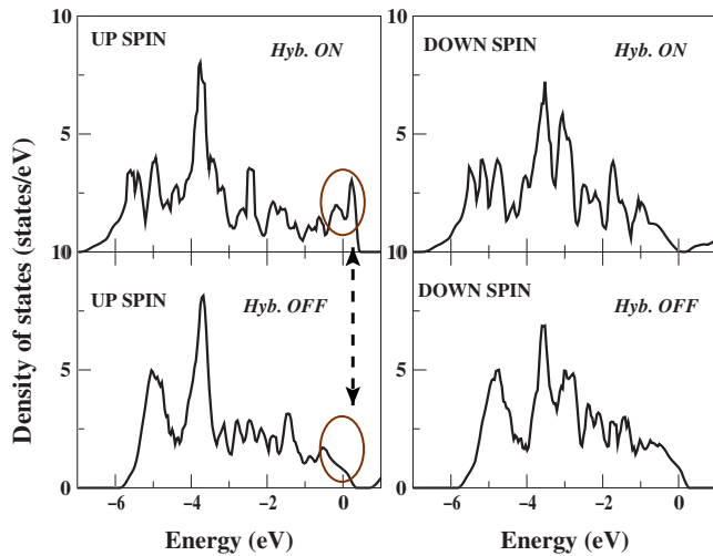
FIG. 3. (Color online) S p density of states of \text{CuCr}_2\text{S}_4 with and without the hybridization between \text{Cr } t_{2g} and the S p - \text{Cu } d hybrid state.
