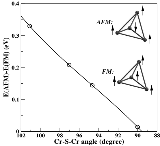
FIG. 1. Total energy difference between AFM and FM spin configurations for a range of \angle Cr-S-Cr, keeping the Cr-S bond length constant in \text{CuCr}_2\text{S}_4 . The inset shows the AFM and FM configuration in a Cr tetrahedral unit.
