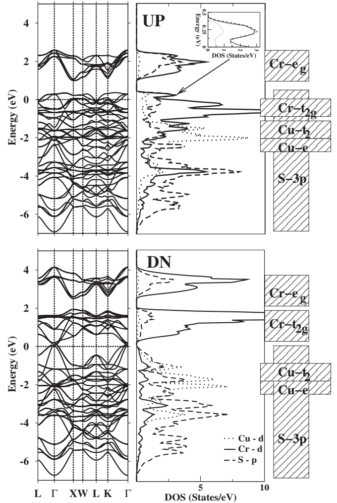
FIG. 2. Left panels show the spin-polarized band structure computed within the local spin density approximation (LSDA) for \text{CuCr}_2\text{S}_4 . The zero of the energy is set at the LSDA Fermi energy E_F . Right panels give the spin-polarized density of states. The inset shows the density of states in the majority spin channel in a small energy range close to E_F .
