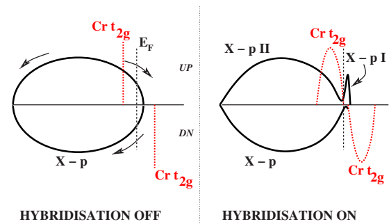
FIG. 4. (Color online) Schematic representation of the exchange mechanism dominant in \text{CuCr}_2\text{X}_4 ( X = \text{S, Se} ).
