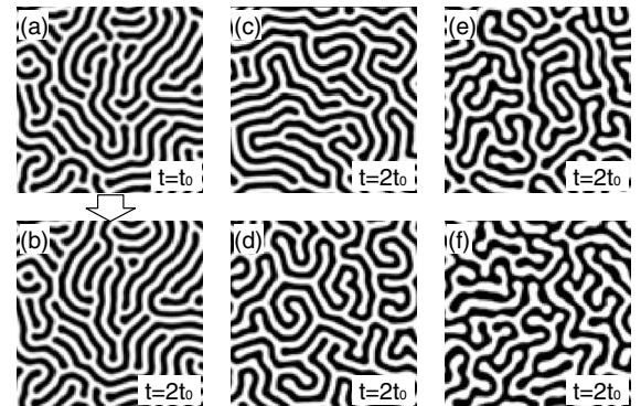
FIG. 4. Domain patterns under zero field after a slow quench ( v=10^{-4} ), which display the dependence on the parameter \alpha : [(a) and (b)] \alpha=1.5 , (c) \alpha=2.0 , (d) \alpha=2.5 , (e) \alpha=3.0 , and (f) \alpha=3.5 . They are the patterns at t=2t_0 except for (a) at t=t_0 .
