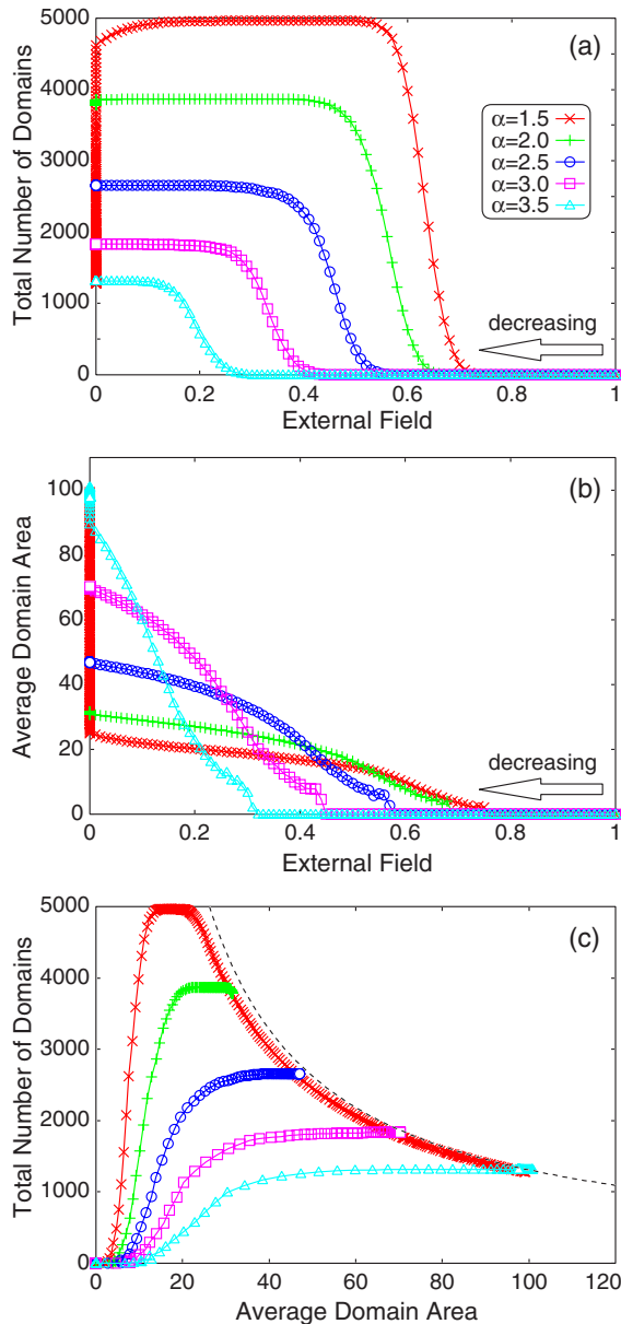
FIG. 2. (Color online) The field dependence of (a) the total number of domains N_{tot} and (b) the average domain area A_{av} ; (c) the A_{av}-N_{tot} graph. The broken line in (c) expresses the curve of A_{av}N_{tot}=512^2/2 , where the total areas of black and white domains are equal. The calculation was performed under a rapidly decreasing field ( v=10^{-2} ) until t=t_0 and then under zero field until t=2t_0 . The number of domains means the number of negative- \phi(r) (black) domains. The domain area is the number of grid points that have negative values of \phi(r) .
