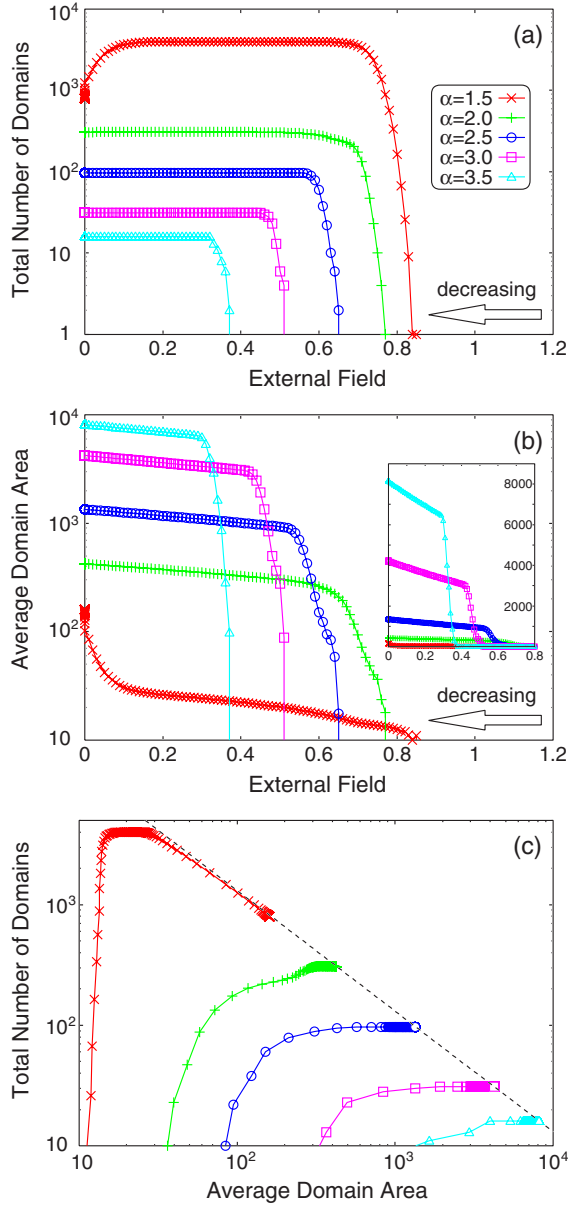
FIG. 5. (Color online) The field dependence of (a) the total number of domains N_{\text{tot}} and (b) the average domain area A_{\text{av}} ; (c) the A_{\text{av}}-N_{\text{tot}} graph. The calculation was performed under a slowly decreasing field ( v=10^{-4} ) until t=t_0 and then under zero field until t=2t_0 . The data are displayed on a semilogarithmic scale in (a) and (b) and on a log-log scale in (c), while the inset of (b) shows the same data as its main panel on a normal scale. The broken line in (c) expresses the curve of A_{\text{av}}N_{\text{tot}}=512^2/2 .
