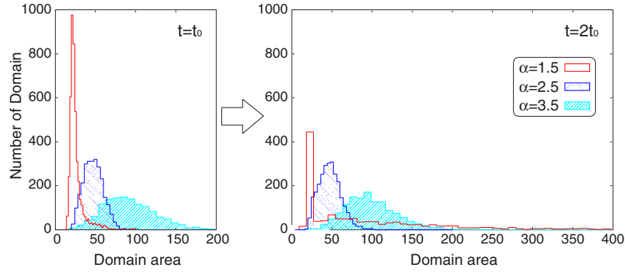
FIG. 3. (Color online) Domain-area distributions at t=t_0 and t=2t_0 . The left, center, and right histograms at each time are for \alpha=1.5 , \alpha=2.5 , and \alpha=3.5 , respectively. The domain area is the number of grid points that have negative values of \phi(\mathbf{r}) .
