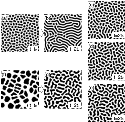
FIG. 1. Domain patterns under zero field after a fast quench ( v=10^{-2} ), which display the dependence on the parameter \alpha : [(a) and (b)] \alpha=1.5 , (c) \alpha=2.0 , (d) \alpha=2.5 , (e) \alpha=3.0 , and [(f) and (g)] \alpha=3.5 . They are the patterns at t=2t_0 except for (a) and (f); these two are the ones at t=t_0 . The size of the snapshots is 96 \times 96 , although the system size is 512 \times 512 . The value of \phi(\mathbf{r}) is positive and negative in the white and black areas, respectively.
