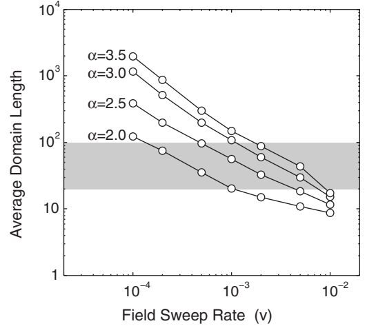
FIG. 6. Dependence of the average domain length at t=2t_0 on the field sweep rate v . The average domain length is calculated from the average domain area and the average domain width (see text). The domain pattern looks like labyrinth and sea-island structures above and below the gray patched area, respectively.
