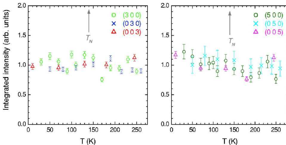
FIG. 4. (Color online) Temperature dependence of the integrated intensity of the (h,0,0) , (0,k,0) , and (0,0,l) , with h, k, l = 3 or 5 reflections on resonance, normalized for comparison.
