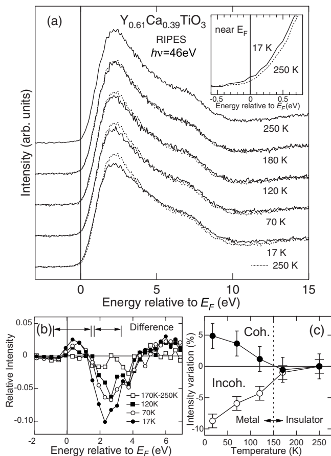
FIG. 7. (a) On-resonance RIPES spectra of Y_{0.61}Ca_{0.39}TiO_3 measured at 17, 70, 120, 180, and 250 K. The spectrum at 250 K is presented by broken lines on each spectrum for comparison. Spectra near E_F are shown in the inset. (b) Difference spectra obtained by subtracting the spectrum at 250 K from that at respective temperatures. (c) Variation of the integrated intensities in the difference spectra for each part of \sim E_F and \sim 2.2 eV (coherent and incoherent parts, respectively) as a function of temperature. The integrated ranges are indicated by horizontal arrows in (b).
