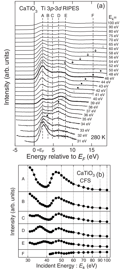
FIG. 2. (a) E_k dependence of RIPES spectra of CaTiO_3 measured at 280 K including the Ti 3p - 3d absorption region. Structures indicated by dots and arrows are the Ca 3d \rightarrow 3p and Ti 3d \rightarrow 3p fluorescence peaks, respectively. (b) CFS spectra of CaTiO_3 for the structures labeled A–F in (a). In the spectrum of A, intensity exhibits the maximum and minimum at E_k=46 and 39 eV, corresponding to the Ti 3p - 3d on- and off-resonances, respectively.
