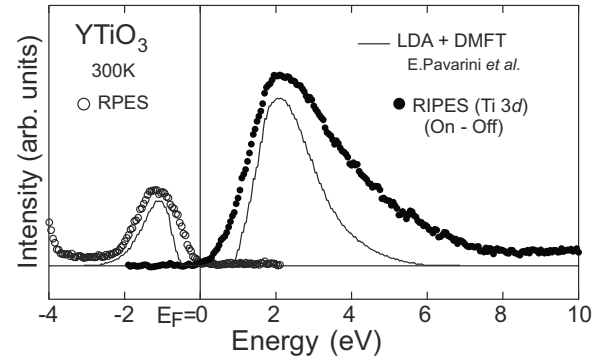
FIG. 5. Comparison of the experimental Ti 3d partial DOS deduced from resonant PES (open circles) and RIPES (closed circles) with the calculated DMFT-DOS (line) (Ref. 36).
