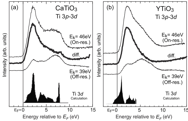
FIG. 4. On- and off-resonance RIPES spectra (thin lines) and the difference spectra (thick lines) of (a) \text{CaTiO}_3 and (b) \text{YTiO}_3 in comparison with the theoretical partial DOS's of Ti 3d states (Refs. 32 and 34).
