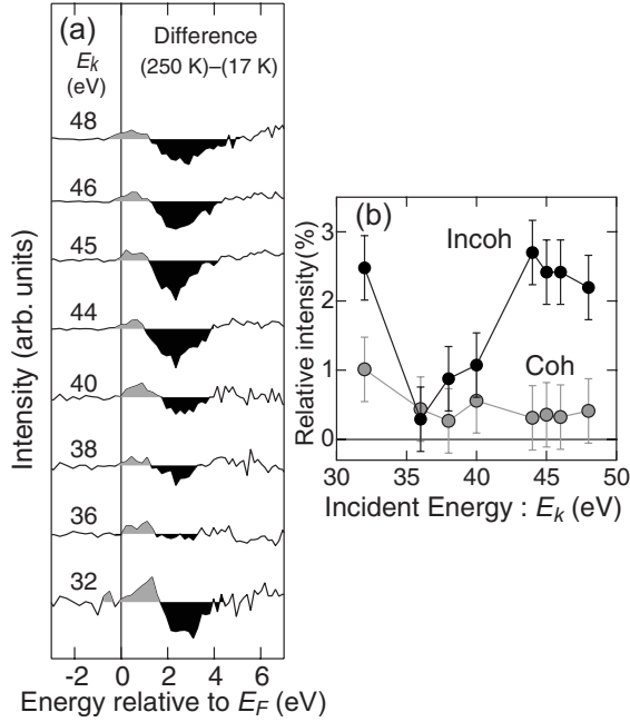
FIG. 8. (a) E_k dependence of difference spectra of Y_{0.61}Ca_{0.39}TiO_3 between 17 and 250 K. In all the spectra, the coherent part (gray) is positive and the incoherent part (black) is negative. (b) Integrated intensities of the coherent (gray) and incoherent (black) parts as a function of E_k .
