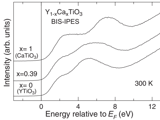
FIG. 1. BIS-IPES spectra of CaTiO_3 , YTiO_3 , and Y_{0.61}Ca_{0.39}TiO_3 measured at 300 K. Emitted photon energy of h\nu=9.4 eV is detected.
