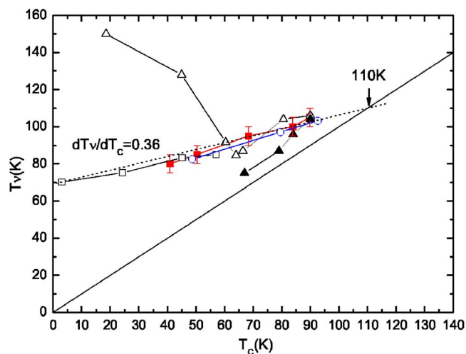
FIG. 6. (Color online) Onset temperature T_\nu of anomalous Nernst signal versus T_c for oxygen-doped and disordered YBCO. Solid square: Pr-YBCO, open triangle: oxygen-doped YBCO (Ref. 16), open square: \text{YBa}_2\text{Cu}_3\text{O}_{6.6} with electron irradiation (Ref. 6), open circle: \text{YBa}_2\text{Cu}_3\text{O}_7 with electron irradiation (Ref. 6), and solid triangle: Zn-YBCO (Ref. 15).
