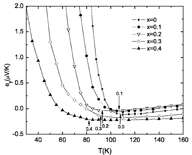
FIG. 4. The temperature dependence of the Nernst signal taken at 14 T for the films. The arrows show the temperatures at which the Nernst signal deviates from the high-temperature background.
