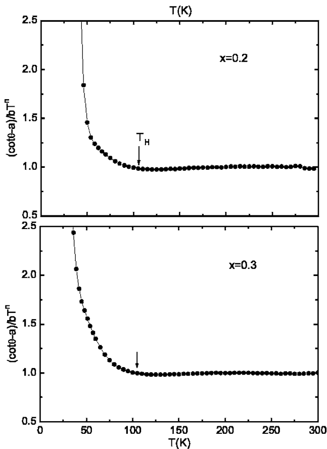
FIG. 2. (\cot \theta - a)/bT^n (see text for details) versus temperature for x=0.2 and 0.3 films. The arrows mark the temperature T_H at which the deviation from the high-temperature behavior starts.
