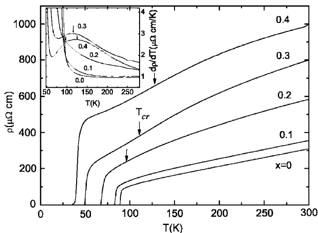
FIG. 1. In-plane resistivity as a function of temperature for the Y_{1-x}Pr_xBa_2Cu_3O_{7-\delta} films ( x from 0 to 0.4). Inset shows the temperature derivative of the resistivity from the main panel for all the films. The arrows indicate the temperature where the peak of the derivative plot appears.
