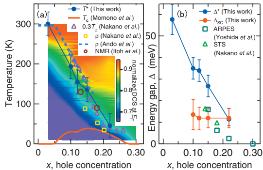
FIG. 3. (Color) Characteristic temperatures (a) and energies (b) in LSCO and LCO. (a) T^* compared with those obtained from the specific heats (Ref. 9), electrical resistivity (Refs. 8 and 9), NMR relaxation time (Ref. 10), and magnetic susceptibility (Ref. 23) and T_c (Ref. 25). The color plot shows the normalized DOS at E_F [ I_{E_F}(x, T) ] and reflects the evolution of the pseudogap in the x - T plane. (b) \Delta^* and \Delta_{sc} compared with the leading edge midpoint in ARPES spectra at \sim(\pi, 0) (Ref. 5) and STS (Ref. 9).
