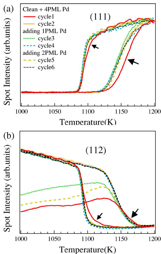
FIG. 7. (Color online) Intensities of LEED spots originated from (a) (111) and (b) {112}-faceted surface as the sample is subjected to three sets of double heating-cooling cycles. Legends of (a) also applies to (b). 4 PML of Pd were deposited onto the surface initially while additional 1 and 2 PML of Pd was deposited in between successive set of double cycles. From (b), one can see that each deposition caused significant change in the intensity of the {112} originated LEED spots. But it is obvious from (a), that there is something special (indicated by the arrows) about the very first annealing cycle after the initial deposition. The transition path for that “virgin” cycle cannot be reproduced by adding additional Pd onto the annealed surface.
