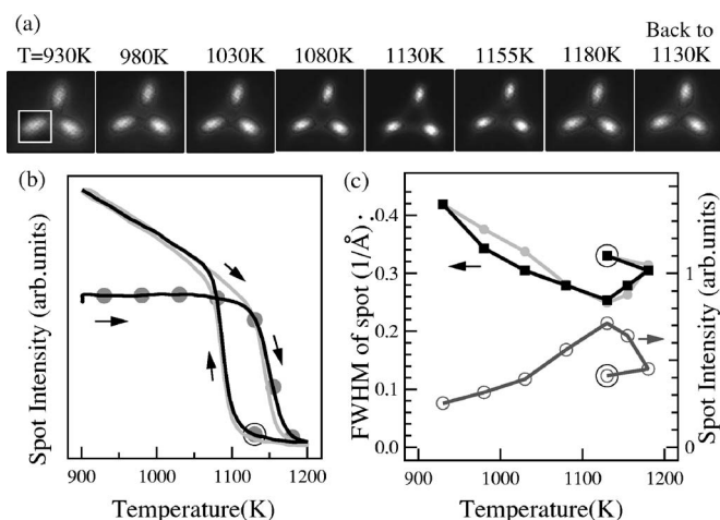
FIG. 5. (a) LEED patterns of a series of samples after they had been annealed at the indicated temperatures for 30 seconds and quenched down to 130 K. The last pattern labeled “back to 1130 K” is of a sample that is first heated to 1200 K and then lowered to 1130 K for annealing. (b) The intensity of a {112} associated LEED spot as a function of temperature during two consecutive annealing cycles is first measured. The annealing temperatures (solid circles) are then selected based on results of the first cycle (the dark curve). (c) The full width at half-maximum W (black solid square) measured along the long axis, and the integrated intensity I (open circle) of the lower left LEED spots shown in (a). The “back to 1130 K” point has been emphasized with a big empty circle. The gray solid circles are plot of \alpha I^{-1/2} . As shown, the width W of the LEED spot is approximately proportional to I^{-1/2} , meaning the facet size are smaller than the transfer width of the LEED electron beam. The lines connecting neighboring data points are guides for the eyes only.
