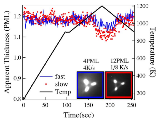
FIG. 4. (Color online) The inset shows the LEED patterns of two samples prepared by either “fast” annealing (4 K/s) or by very “slow” annealing (1/8 K/s). The figure shows the apparent thickness of the two samples as functions of time when undergoing identical subsequent annealing processes (4 K/s).
