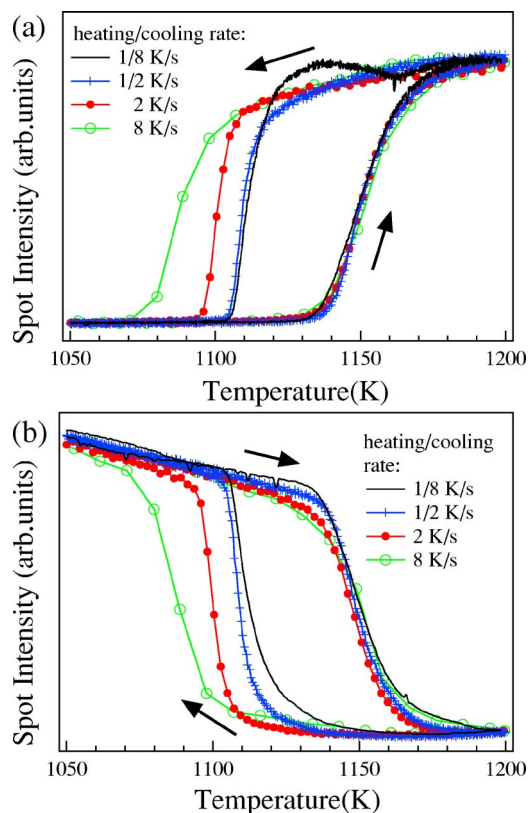
FIG. 8. (Color online) Intensities of the LEED spots associated with (a) (111) and (b) {112}-faceted surface are plotted as functions of temperature for samples subjected to different heating-cooling rates (see text for detail). Note the negligible dependence of the transition paths on the heating rate for the defaceting transitions, in contrast with the strong dependence of the paths on the cooling rate for the faceting transitions.
