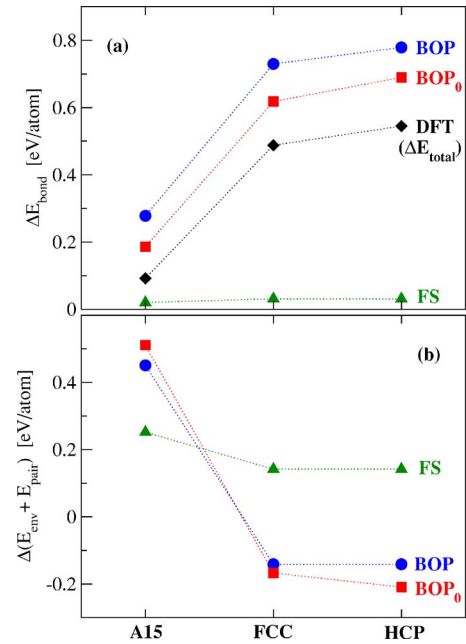
FIG. 5. (Color online) Comparison of E_{bond} (a) and E_{env} + E_{pair} (b) contributions to the structural energy differences between various close-packed structures and the bcc structure, calculated by BOP, BOP 0 , and FS. (a) also contains the total energy differences obtained from DFT calculations.
