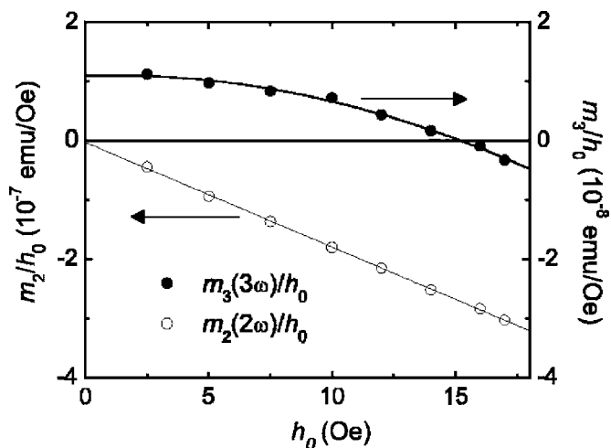
FIG. 1. Illustration of the method employed for measuring the nonlinear susceptibilities (here T=8 K, H_z=100 Oe, and \omega/2\pi=2 kHz). \chi_2(2\omega) and \chi_3(3\omega) are obtained, respectively, from the slope and the quadratic coefficient of the second m_2(2\omega)/h_0 and third m_3(3\omega)/h_0 harmonics of the output signal, measured as a function of the ac field amplitude h_0 .
