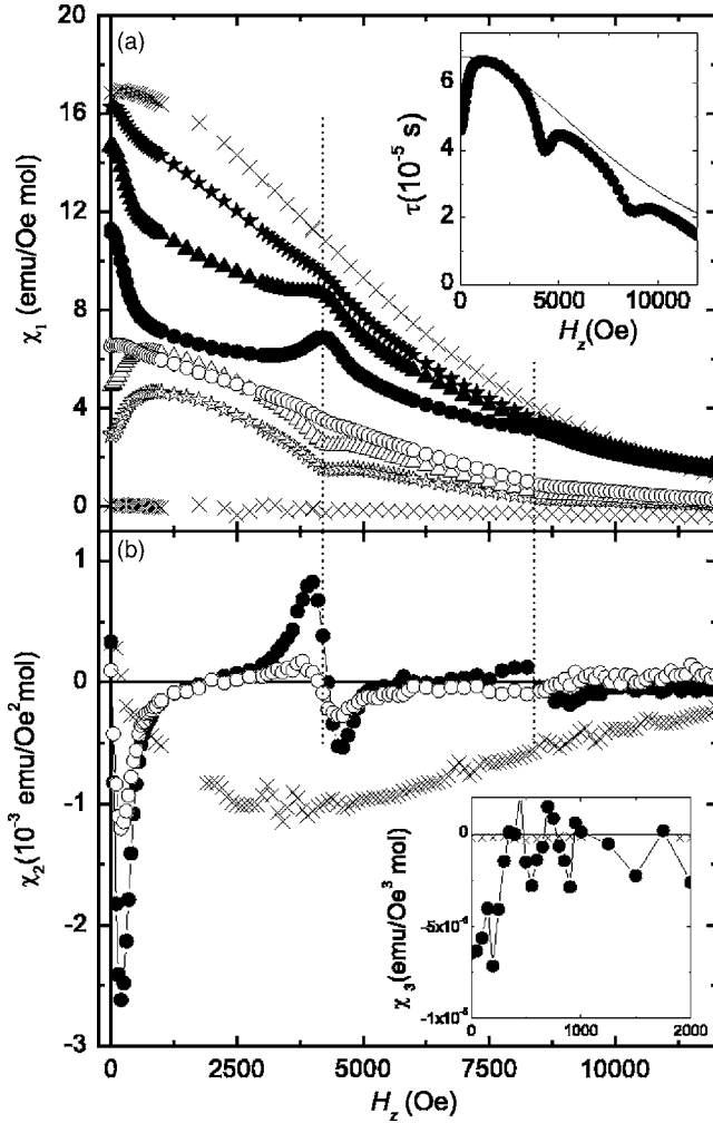
FIG. 2. (a) Linear susceptibility of \text{Mn}_{12} measured at T=8 K versus a magnetic field applied parallel to the anisotropy axis. \times , \omega/2\pi=1 Hz ( \sim equilibrium); \star , 500 Hz; \Delta , 1 kHz; \bullet , 2 kHz. Solid symbols, real parts; open symbols, imaginary parts. The inset shows the relaxation time \tau , as obtained from \chi_1''/\omega\chi_1' [see Eq. (1)] as well as calculated for classical spins (line) (Ref. 14). (b) Second harmonic susceptibility measured at the same temperature. \bullet and \circ , \chi_2'(2\omega) and \chi_2''(2\omega) at 2 kHz; \times , equilibrium \chi_2^{\text{eq}}=(d\chi_1^{\text{eq}}/dH_z)/2 . Inset: \bullet , \chi_3'(3\omega) at 2 kHz; \times , \chi_3^{\text{eq}}=(d^2\chi_1^{\text{eq}}/dH_z^2)/6 . The dotted vertical lines mark the resonant fields H_1 \approx 4200 Oe and H_2=2H_1 .
