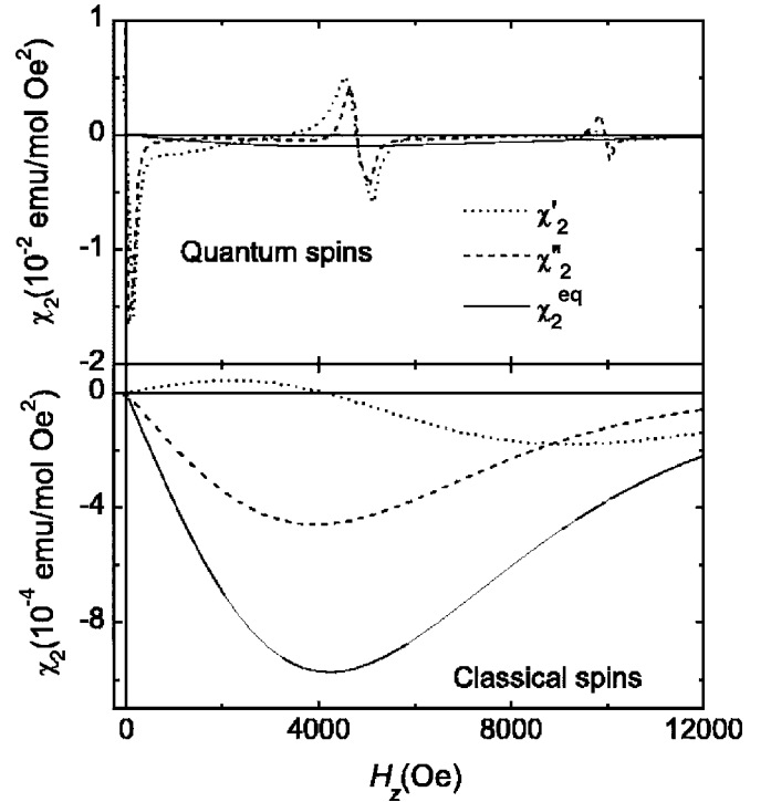
FIG. 3. Theoretical calculations of \chi_2(2\omega) [Eq. (2)] for quantum and classical spins. In the latter case, we used Brown’s classical formula for \tau (Ref. 14) and in the former \tau was calculated by solving Pauli’s quantum master equation, as described in Ref. 16. Notice the difference in the \chi_2 axis scale (the solid equilibrium curve is the same in both panels).
