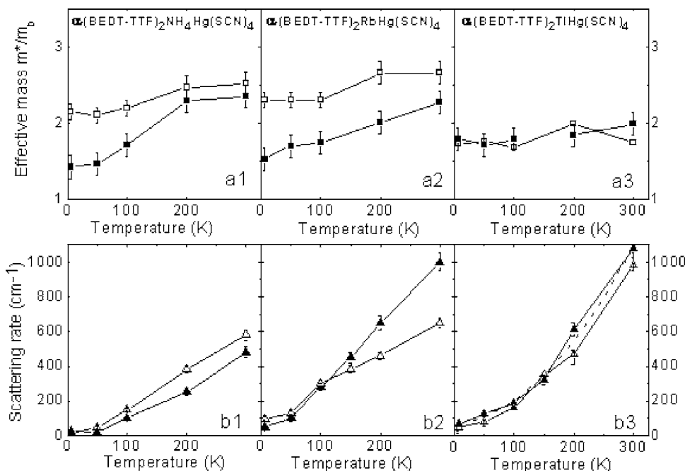
FIG. 6. Temperature dependence of the m^*/m_b (upper panel) and Drude-scattering rate \gamma (lower panel) for \alpha -(BEDT-TTF) _2 MHg(SCN) _4 ( M =NH _4 , Rb, Tl) compounds. Filled squares: E_{\perp} stacks, empty squares E_{\parallel} stacks. For the Tl salt a \gamma \sim T^2 fit of the scattering rate is shown with a dashed line.
