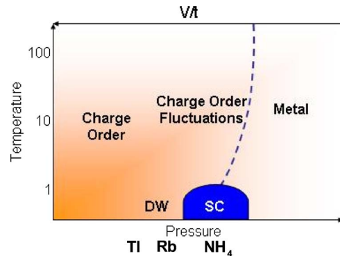
FIG. 8. (Color online) Phase diagram for the quarter-filled two-dimensional organic conductors \alpha -(BEDT-TTF) _2 MHg(SCN) _4 ( M = \text{NH}_4, \text{K}, \text{Rb}, \text{TI} ). With increasing pressure the effective intersite Coulomb repulsion V/t is reduced. At intermediate temperatures the system is tuned from a charge-order (CO) state to a metal with charge fluctuations in between. We propose that the compounds with M = \text{K}, \text{TI} are to be found in this part of the phase diagram. We propose that the Rb salt has lower influence of correlations, and the NH _4 salt is even less correlated, distinctly showing the increase of metallic properties on cooling, and becoming superconducting (SC) below 1 K.
