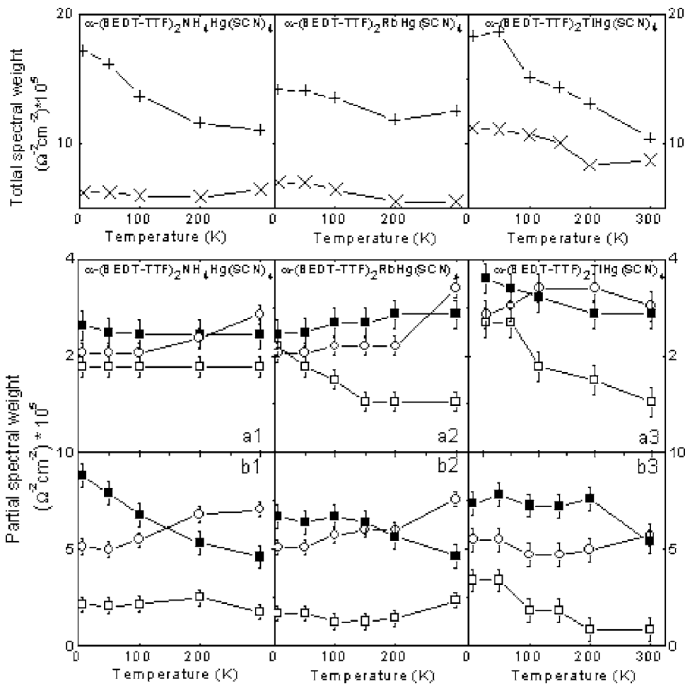
FIG. 5. Upper panel: temperature dependence of the total spectral weight for \alpha -(BEDT-TTF) _2 MHg(SCN) _4 ( M =NH _4 , Rb, Tl) parallel to the stacks (diagonal crosses) and perpendicular to the stacks (straight crosses). Lower panel: Temperature dependence of the spectral weight for the three main features in the optical spectra of \alpha -(BEDT-TTF) _2 MHg(SCN) _4 ( M =NH _4 , Rb, Tl) compounds. Filled squares: Drude peak, empty squares: 1000 \text{cm}^{-1} maximum, empty circles: 2500 \text{cm}^{-1} maximum. (a) Polarization parallel to the stacks direction and (b) perpendicular to the stacks. Note different scales for the different contributions and polarizations.
