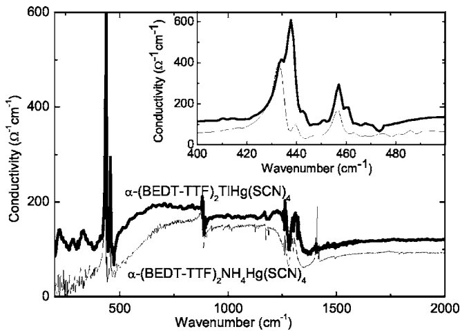
FIG. 7. The T=6 K spectra of \alpha -(BEDT-TTF) _2 TIHg(SCN) _4 (thick line) and \alpha -(BEDT-TTF) _2 NH _4 Hg(SCN) _4 (thin line) in E_{||} stacks polarization. The inset shows the spectral range with \nu_{12}(A_g) and \nu_{13}(A_g) EMV-coupled features for these two spectra. For \alpha -(BEDT-TTF) _2 TIHg(SCN) _4 to electronic band at 1000 \text{cm}^{-1} has higher intensity, and the vibrational features are split, pointing on an ordered state.
