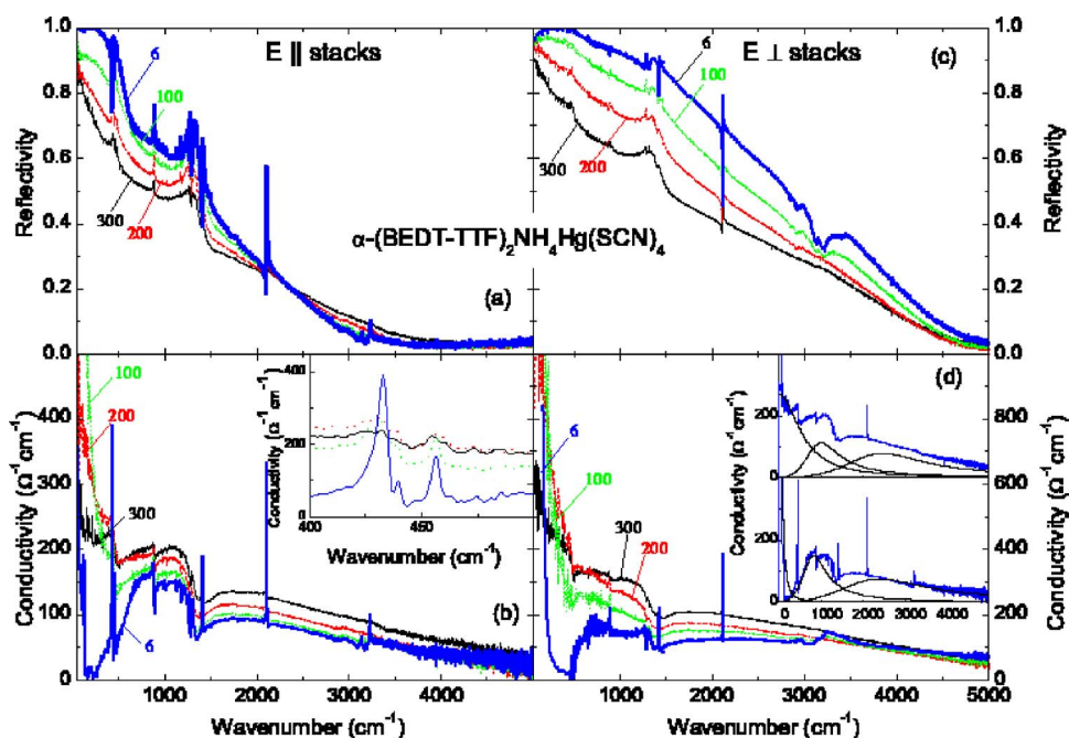
FIG. 1. (Color online) Reflectivity and conductivity spectra of \alpha -(BEDT-TTF) _2 NH _4 Hg(SCN) _4 at T=300, 200, 100, and 6 K; left panels (a) and (b): E \parallel stacks, right panels (c) and (d): E \perp stacks. The insets show optical conductivity in the range of \nu_{12}(A_g) and \nu_{13}(A_g) modes. The inset in (d) shows the contributions of one Drude and two Lorentz components for E \parallel stacks 300 and 6 K.
