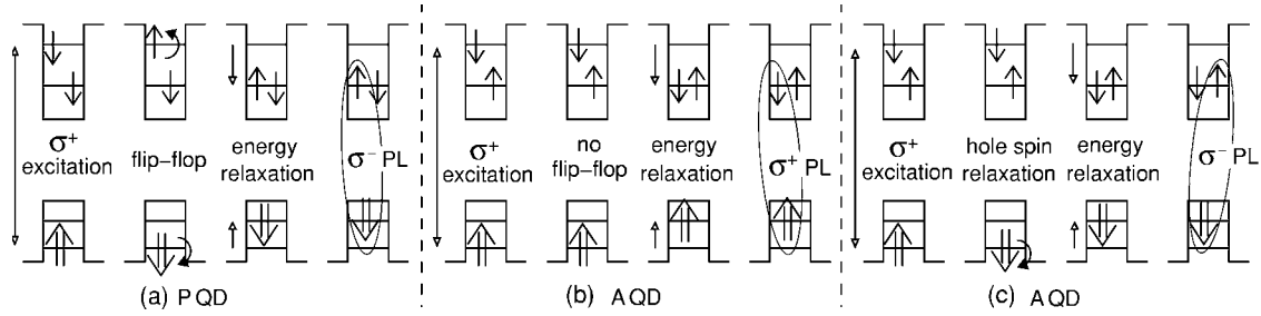
FIG. 2. Schematic spin orientation of electrons and a hole in a quantum dot, after circularly polarized photoexcitation generates an electron-hole pair at the excited state in a single-electron-doped quantum dot. (a) A process to generate negative circularly polarized luminescence in a PQD. PQD denotes a quantum dot in which the spin of the doped electron is oriented parallel to the helicity of the circularly polarized excitation. (b) A process to generate positive circularly polarized luminescence in an AQD. AQD denotes a quantum dot in which the spin of the doped electron is oriented antiparallel to the helicity of the circularly polarized excitation. (c) Spin flip of a single particle-hole in an AQD, which causes optical pumping of the doped electron.
