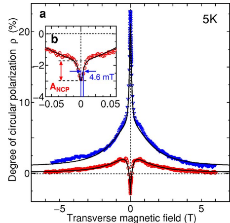
FIG. 3. (Color online) (a) Hanle curves for InP QDs at 5 K under -0.1 V. The excitation photon energy was 1.771 eV (circles) or 1.746 eV (triangles) and the detection energy was 1.722 eV. A sum of three Lorentzians is used in the fit of the lower Hanle curve, while a sum of two Lorentzians is used in the fit of the upper Hanle curve. The narrowest Lorentzian dip observed in the lower Hanle curve for the excitation at 1.771 eV has half width at half maximum of 4.6 mT as shown in (b).
