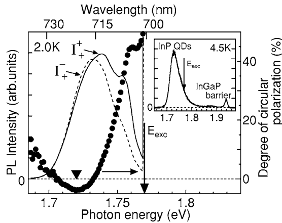
FIG. 1. Circularly polarized photoluminescence spectra of InP quantum dots at 2.0 K under selective circularly polarized excitation of the dots at 1.771 eV, below the \text{In}_{0.5}\text{Ga}_{0.5}\text{P} barrier band gap. The electric bias applied is -0.1 V. Degree of circular polarization of PL is shown by solid circles. The shoulder seen at the excitation-detection energy difference of \Delta E = 10 meV can be ascribed to the transverse acoustic phonon structure. In the inset, the PL spectrum of the sample under green laser excitation at 2.33 eV is shown and the excitation photon energy of 1.771 eV for the circularly polarized PL experiment is indicated by an arrow.
