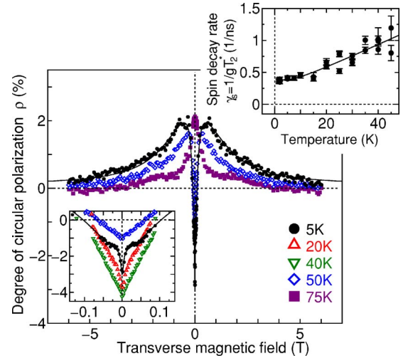
FIG. 5. (Color online) Hanle curve vs temperature under -0.1 V bias. The excitation photon energy was 1.771 eV and the detection photon energy was 1.722 eV. The lower inset shows that the sharpest first Lorentzian component broadens and fades away at elevated temperature. The upper figure shows the temperature dependence of the spin dephasing rate \gamma_s=1/gT_2^* deduced from the sharpest Lorentzian width as a function of temperature.
