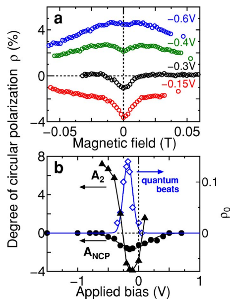
FIG. 4. (Color online) (a) The sharpest Hanle dip vs the electric bias. (b) Closed circles fitted by a Gaussian with full width at half maximum of \Delta U = 0.46 V show the amplitude of the sharp (first) Lorentzian component. Open diamonds show the amplitude of the measured trionic quantum beat. Triangles show Lorentzian fitting parameter A_2 for Hanle curves vs the electric bias. Peak (dip) positions of the three fitting lines are in accord.
