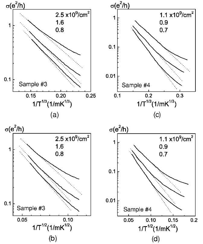
FIG. 3. Comparison of the conductivities \sigma(T) with VRH transport models: (a), (c) Mott and (b), (d) Efros-Shklovskii. Panels (a) and (b) are results from sample No. 3, and (c) and (d) are from sample No. 4.
