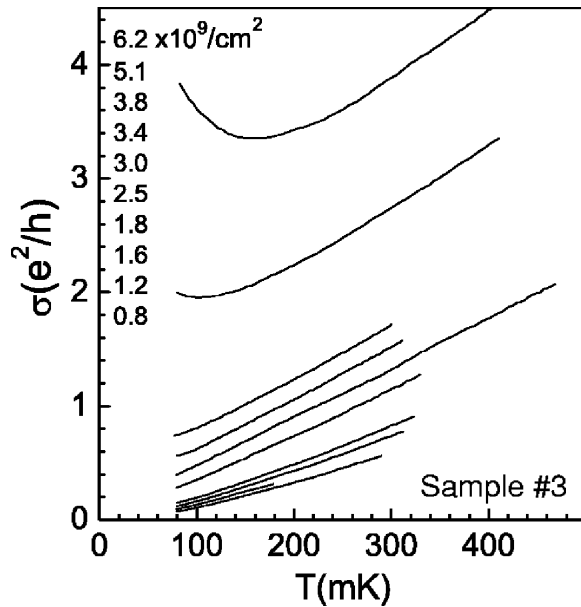
FIG. 2. Re plot of the data from Fig. 1 in terms of conductivity vs temperature.
