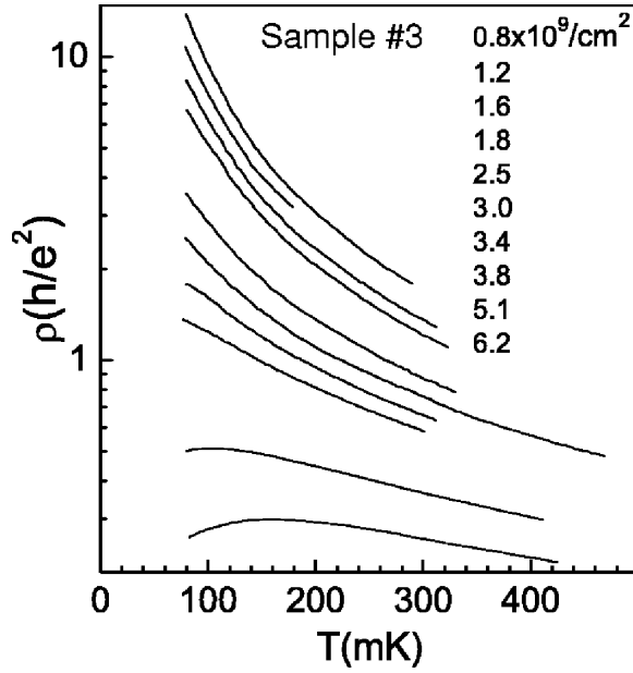
FIG. 1. Temperature dependence of the resistivity of sample No. 3 in semilogarithmic scale for a set of specified hole densities listed on the right-hand side.
