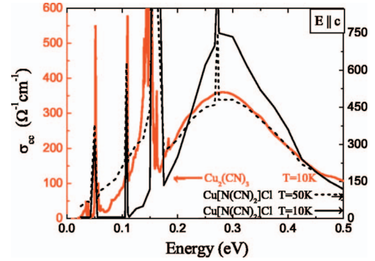
FIG. 4. (Color) Comparison of the low-temperature optical conductivity of \kappa -(ET) _2 Cu _2 (CN) _3 and \kappa -(ET) _2 Cu[N(CN) _2 ]Cl. For the former compound, the T = 10 K spectrum representative for the whole T < 100 K range is only displayed. The conductivity spectra for \kappa -(ET) _2 Cu[N(CN) _2 ]Cl are reproduced from Ref. 24. The left (right) scale corresponds to \kappa -(ET) _2 Cu _2 (CN) _3 ( \kappa -(ET) _2 Cu[N(CN) _2 ]Cl).
