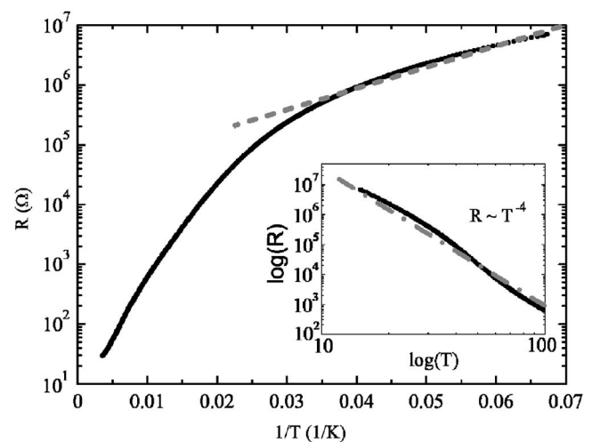
FIG. 1. Arrhenius plot of the resistance of a \kappa -(ET) 2 Cu 2 (CN) 3 single crystal. The gray dashed line at low temperature indicates the fitting of the gap value according to R(T)=R_0 \exp(\Delta/2k_B T) . Inset: \log(R) vs \log(T) plot indicative of a power-law behavior of the resistance in the low-temperature region.
