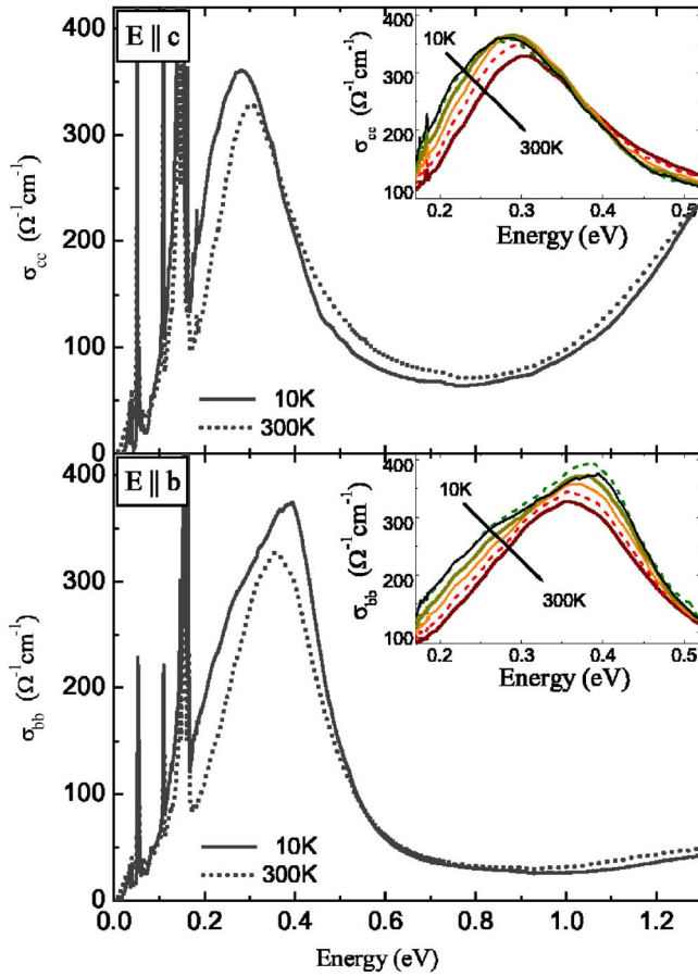
FIG. 3. (Color online) Optical conductivity spectra of \kappa -(ET) _2 Cu _2 (CN) _3 at the lowest and highest temperature of the measurement for E \parallel c and E \parallel b shown in the upper and lower panel, respectively. The temperature evolution of the dimer peak is enlarged in the insets.
