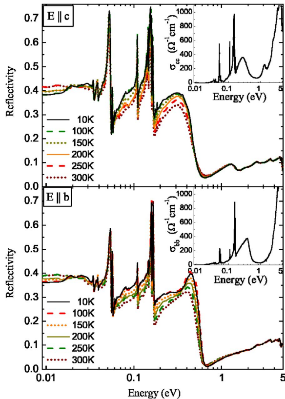
FIG. 2. (Color online) Polarized reflectivity spectra of \kappa -(ET) _2 Cu _2 (CN) _3 measured at various temperatures for E\parallel c and E\parallel b (upper and lower panel, respectively). The insets show the corresponding conductivity spectra at low temperature.
