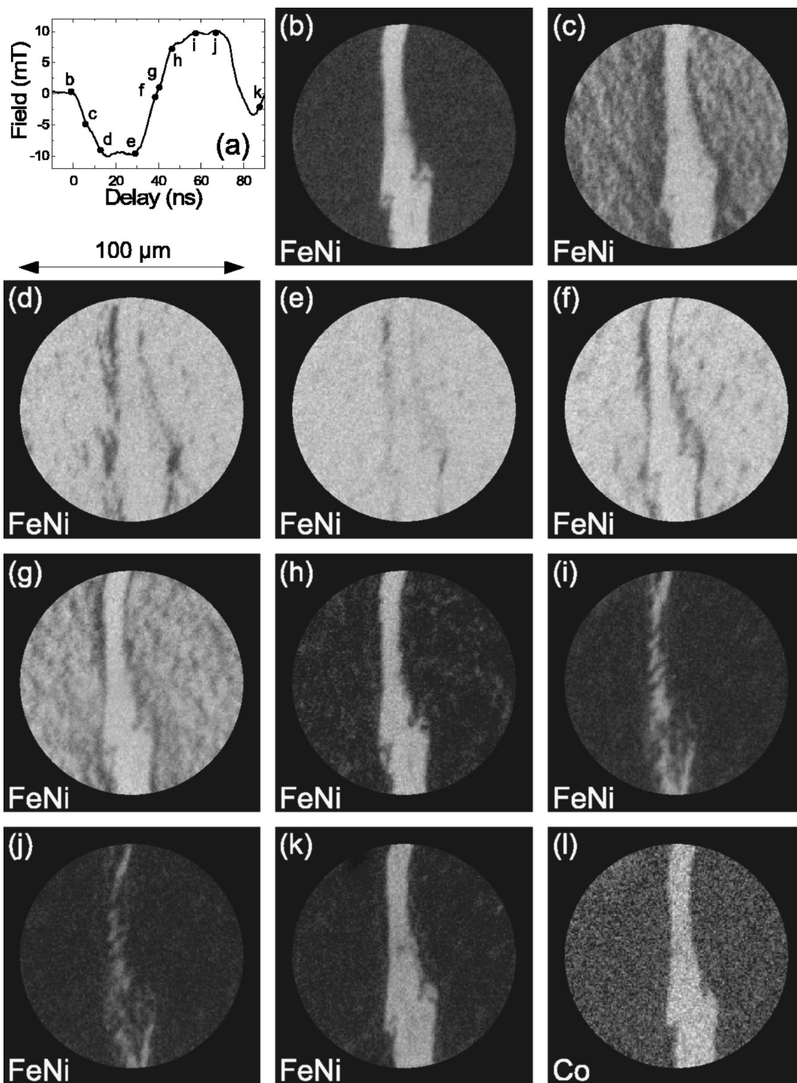
FIG. 5. Time-resolved PEEM images for sample I ( 4^\circ miscut angle). (a) Bipolar applied magnetic field pulses. (b)–(k) FeNi domain structure for different delays between magnetic field and photon pulses as indicated in (a). (l) Co domain structure. The directions of incoming photons, applied field, and local magnetization are the same as in Fig. 4. The field of view for each image is 100 \mu\text{m} .
