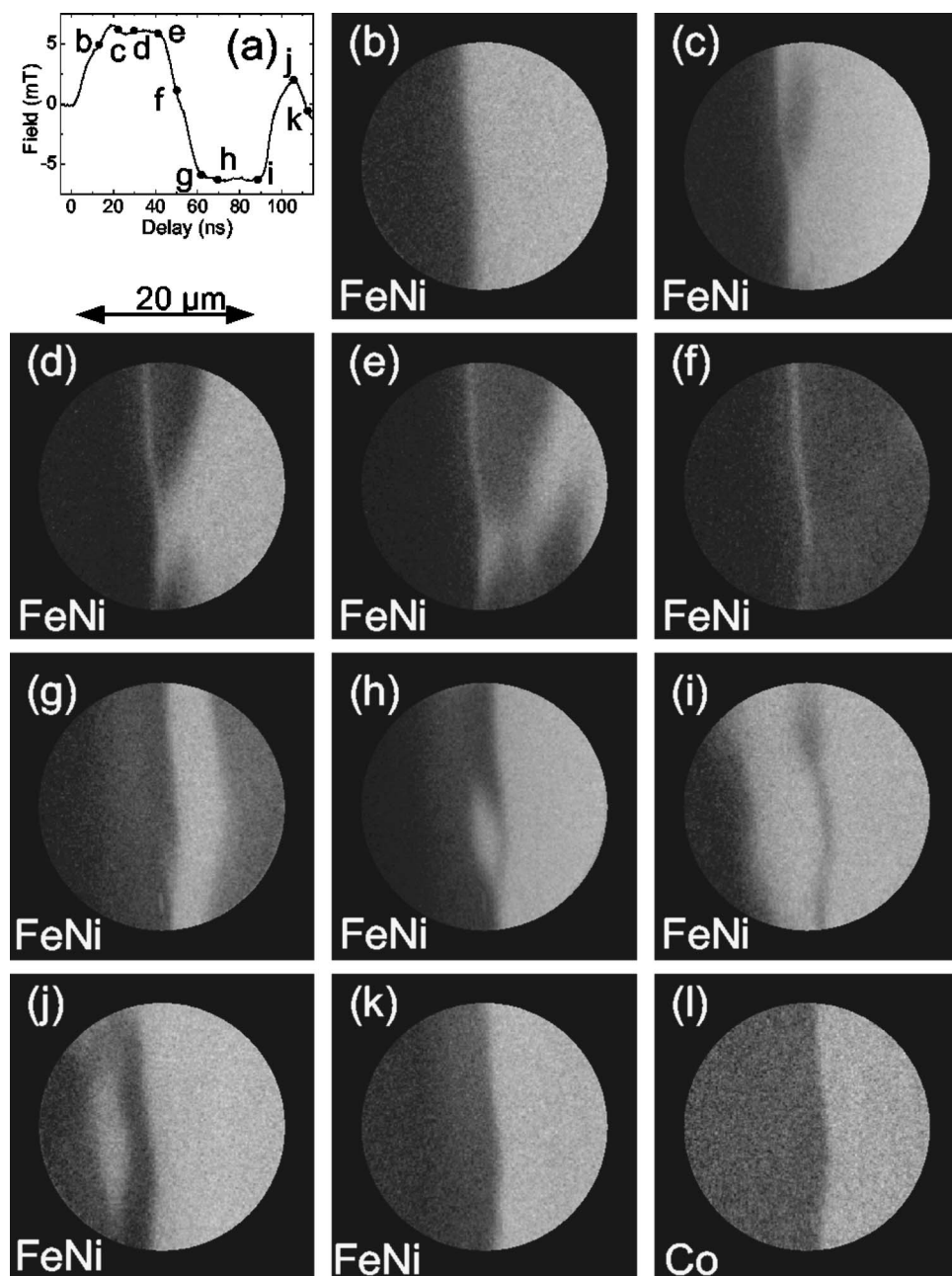
FIG. 7. Time-resolved PEEM images for sample III ( 8^\circ miscut angle). (a) Bipolar applied magnetic field pulses. (b)–(k) FeNi domain structure for different delays between field pulse and photon pulses as indicated in (a). (l) Co domain structure. The directions of incoming photons, applied field, and local magnetization are the same as in Fig. 4. The field of view for each image is 20 \mu\text{m} .
