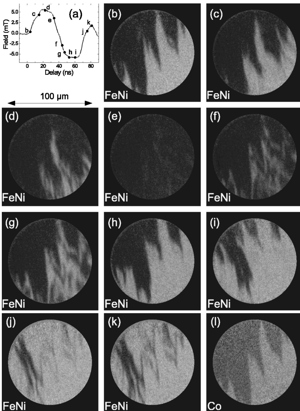
FIG. 6. Time-resolved PEEM images for sample II ( 6^\circ miscut angle). (a) Bipolar applied magnetic field pulses. (b)–(k) FeNi domain structure for different delays between field pulse and photon pulses as indicated in (a) (l) Co domain structure. The directions of incoming photons, applied field, and local magnetization are the same as in Fig. 4. The field of view for each image is 100 \mu\text{m} .
