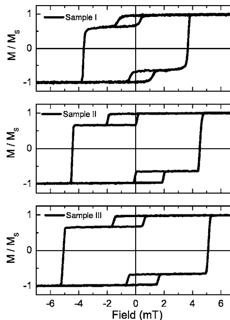
FIG. 1. Quasistatic hysteresis loops and minor loops for magnetic tunnel junctions deposited on step-bunched Si with a miscut angle of 4^\circ (top), 6^\circ (middle), and 8^\circ (bottom). The hysteresis loops are taken with the magnetic field applied along the easy magnetization axis (parallel to the long axis of the substrate terraces).
