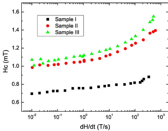
FIG. 2. (Color online) Coercive field of the Fe 20 Ni 80 layer as a function of the applied field sweep rate dH/dt .
