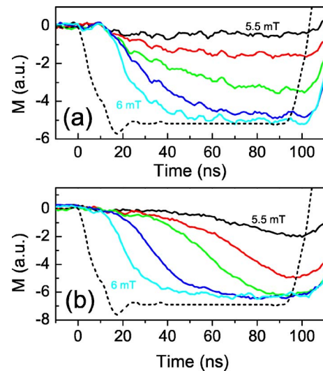
FIG. 3. (Color online) Fast magnetization relaxation for sample II (a) and sample III (b). The magnetization decay is plotted as solid lines for different applied field values between 5.5 and 6 mT. The shape of the magnetic field pulse for a pulse with an amplitude of 6 mT is shown as the dashed line. A synchronous noise can be seen in (a). This noise is due to electromagnetic interference created by the current generator and the coil.
