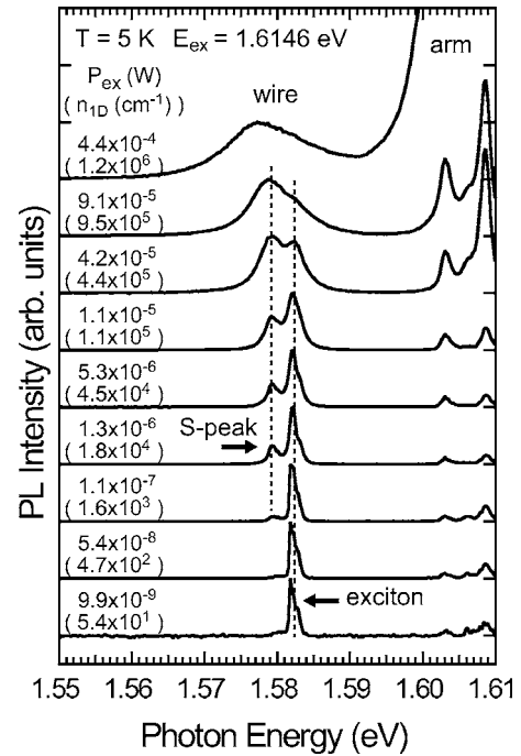
FIG. 5. Normalized PL spectra of the T wire for various excitation powers ( P_{ex} ) at 5 K. Numbers in parentheses are estimated 1D e-h pair densities ( n_{1D} ). The low-energy side peak that appeared below the wire exciton peak is labeled as the S-peak. Two dashed vertical parallel lines are drawn to guide the eyes. PL peaks observed above 1.60 eV were from the arm wells.
