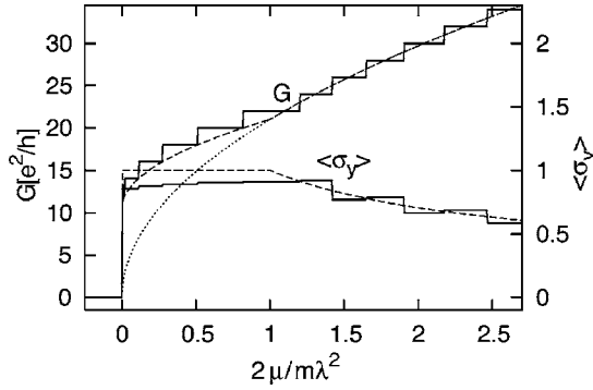
FIG. 1. Conductance (in units of e^2/h ), and spin polarization of the current vs gate voltage (in units of m\lambda^2/2 ). Dashed lines show the smoothed curves (14) and (15), solid lines show the quantized values for m\lambda L/\hbar = 10.5\pi . Dotted line shows the conductance without spin-orbit interaction.
