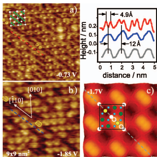
FIG. 3. (Color) STM constant current scans taken subsequently from the same area at -0.73 \text{ V} (a) and -1.85 \text{ V} (b) sample bias and theoretical STM image of the dimeric A termination at negative ( V_s = -1.7 \text{ V} ) sample bias (c). Small circles in (a) mark positions of atoms that are equivalent to oval contours in (b). The experimental height profiles along \langle 110 \rangle , with colors corresponding to lines marked in (a) and (b), and the theoretical one in gray are shown in the upper right plot. Circle models in (a) and (c) indicate atomic positions on an ideal surface with tetrahedral termination. Green circles represent surface octahedral Fe atoms arranged in rows along \langle 110 \rangle , filled white circles are surface tetrahedral Fe atoms in their bulklike positions arranged in the (1 \times 1) square lattice, open white circles are surface tetrahedral irons in dimers, yellow circles are subsurface tetrahedral Fe atoms, and small blue circles are oxygen atoms.
