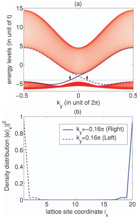
FIG. 2. (Color online) (a) Energy spectrum of the QAHE system (7) when the open boundary condition is imposed in x -direction. The parameters are c=1, t/V=1/3, e_s=0.5 . The solid and dashed lines between two energy bands stand for the edge states at the right and left edge, respectively. The horizontal dotted line shows a typical chemical potential inside the gap. The two arrows mark the two gapless edge excitation with momentum k_y = \pm 0.16\pi . (b) the density distribution of the two edge states at fermi surface, calculated for a 50 \times 50 lattice.
