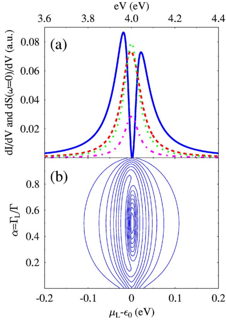
FIG. 1. (Color online) Conductance and differential noise vs applied source-drain voltage. (a) dS(\omega=0)/dV (solid and dashed lines) and dI/dV (dotted and dash-dotted lines) for \alpha=0.5 and \alpha=0.1 , respectively. (b) Contour plot of dS(\omega=0)/dV . See text for units.
