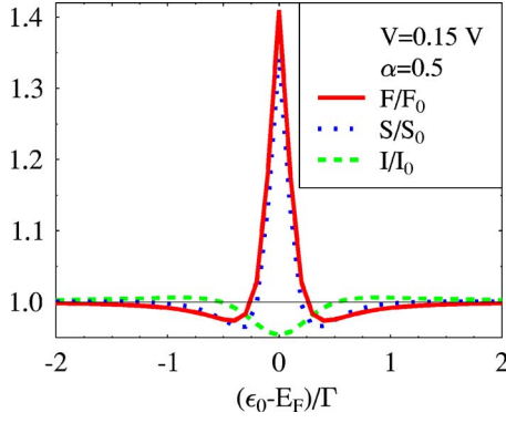
FIG. 7. (Color online) Ratios of Fano factors (solid line), zero frequency noises (dotted line), and currents (dashed line) with and without electron-phonon coupling vs position of the molecular orbital relative to the Fermi energy. See text for parameters.
