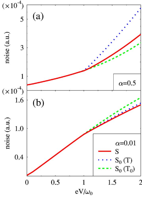
FIG. 3. (Color online) Zero frequency noise with (solid line) and without (dashed line) electron-phonon interaction for (a) symmetric, \alpha=0.5 , and (b) asymmetric, \alpha=0.01 molecule-leads coupling in the resonant tunneling regime. Also shown is approximate result (dotted line) where noise is calculated as a sum of thermal and shot noise, Eqs. (20)–(22), with renormalized transmission coefficient T , Eq. (38), replacing the elastic tunneling transmission T_0 , Eq. (23). See text for parameters.
