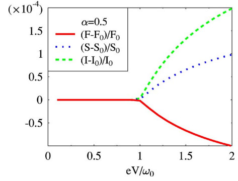
FIG. 6. (Color online) Ratios of Fano factors (solid line), zero frequency noises (dotted line), and currents (dashed line) with and without electron-phonon coupling vs applied voltage in the off-resonant tunneling regime. See text for parameters.
