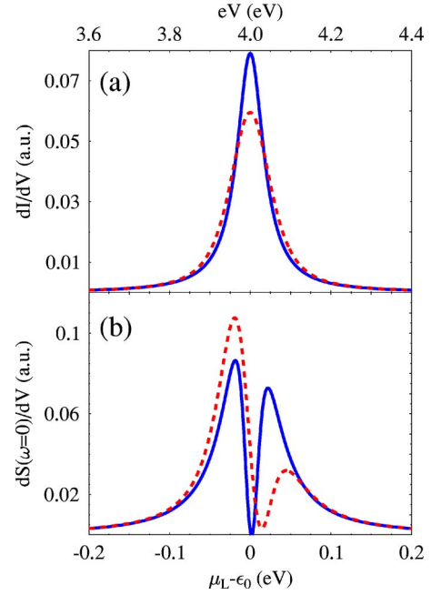
FIG. 2. (Color online) Conductance (a) and differential noise (b) vs applied source-drain voltage. Shown are results for T=10 K (solid line) and T=100 K (dashed line).
