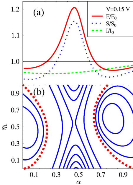
FIG. 5. (Color online) (a) Ratios of Fano factors ( F/F_0 , solid line), zero frequency noises ( S/S_0 , dotted line), and currents ( I/I_0 , dashed line) with and without electron-phonon coupling vs asymmetry in coupling to the leads in the resonant tunneling regime. \eta_L=0.5 (b) F/F_0 a function of two asymmetry parameters, \alpha and \eta_L in the resonant tunneling regime. Dotted line represents F/F_0=1 case. Parameters are the same as in Fig. 4 and the voltage bias is V=0.15 V ( eV=1.5\hbar\omega_0 ).
