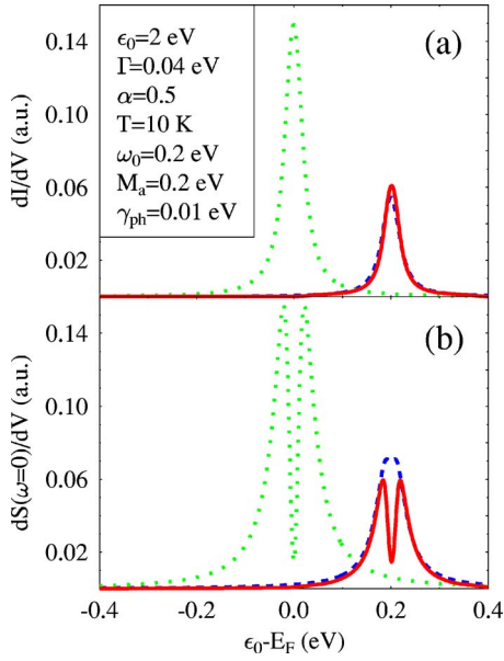
FIG. 8. (Color online) Conductance (a) and differential noise (b) vs level position (gate voltage experiment). Shown are results of self-consistent calculation (solid line) and the zero order approximation (dashed line). Results in the absence of electron-phonon coupling (dotted line) are given for comparison.
