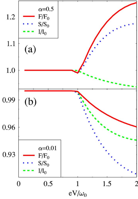
FIG. 4. (Color online) Ratios of Fano factors (solid line), zero frequency noises (dotted line), and currents (dashed line) with and without electron-phonon coupling vs applied voltage in the resonant tunneling regime. Shown are (a) symmetric \alpha=0.5 and (b) asymmetric \alpha=0.01 coupling case. Parameters are the same as in Fig. 3.
