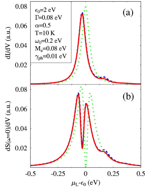
FIG. 9. (Color online) Conductance (a) and differential noise (b) vs applied source-drain voltage for the case of relatively weak electron-phonon coupling. The different lines represent results for the full and zero order calculation and for the case with no electron-phonon coupling (line notation as in Fig. 8).
