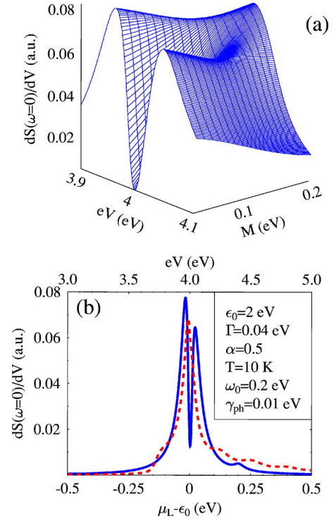
FIG. 11. (Color online) Differential noise vs applied source-drain voltage for \alpha=0.5 . (a) Surface plot of dS(\omega=0)/dV as function of source-drain voltage and electron-phonon coupling strength. Zero-order result. (b) dS(\omega=0)/dV for weak ( M=0.04 eV, solid line) and strong ( M=0.3 eV, dashed line) electron-phonon coupling. Self-consistent calculation.
