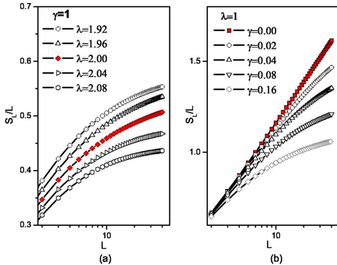
FIG. 4. (Color online) Scaling of the block entropy S_L in d=2 for \gamma=1 (left panel) and \lambda=1 (right panel).
