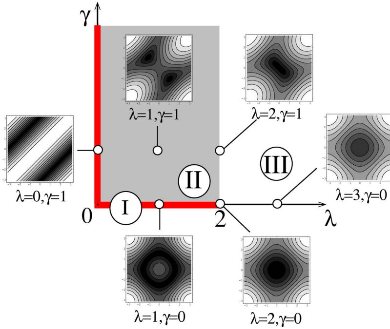
FIG. 1. (Color online) Phase diagram of the model, Eq. (2), for the case d=2 . The roman numbers for the various phases are explained in the text. Representative contour plots of the dispersion relation \Lambda_k are also shown. There the black areas corresponds to \Lambda_k=0 and the white areas to the top of the band.
