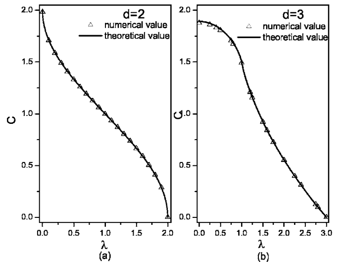
FIG. 3. \lambda dependence of the C coefficient in Eq. (1) in d=2 and d=3 . The values extracted from fits to our numerical data are compared with the predictions of Ref. 16. In d=2 , the exact form of C(\lambda) can be obtained, which is equal to \frac{2}{\pi} \cos^{-1}(\lambda-1) .
