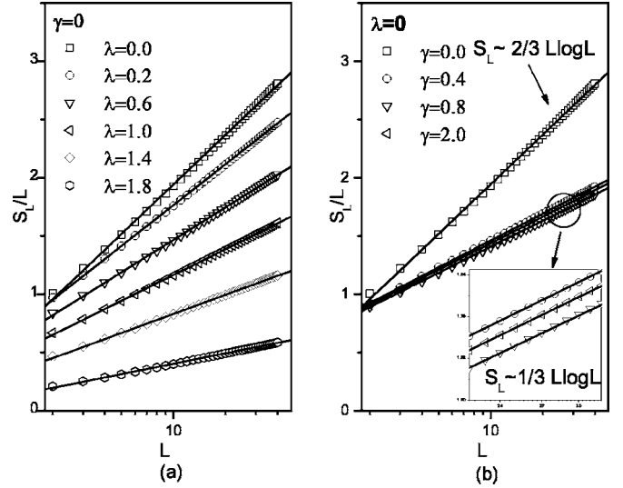
FIG. 2. Scaling of the block entropy S_L in d=2 for \gamma=0 (left panel) and \lambda=0 (right panel). The solid lines correspond to fits according to the formula S_L = \frac{C}{3} L \log_2(L) + BL + A .
