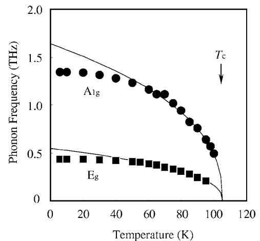
FIG. 5. Temperature dependence of the oscillation frequency obtained from the coherent phonon signal below T_c . The solid circles are the oscillation frequency for the A_{1g} mode, and the solid squares are that for the E_g mode. The solid curves describe a temperature dependence of the form \omega \propto (T_c - T)^n , where T_c = 105 K and n = 0.4 for both modes.
