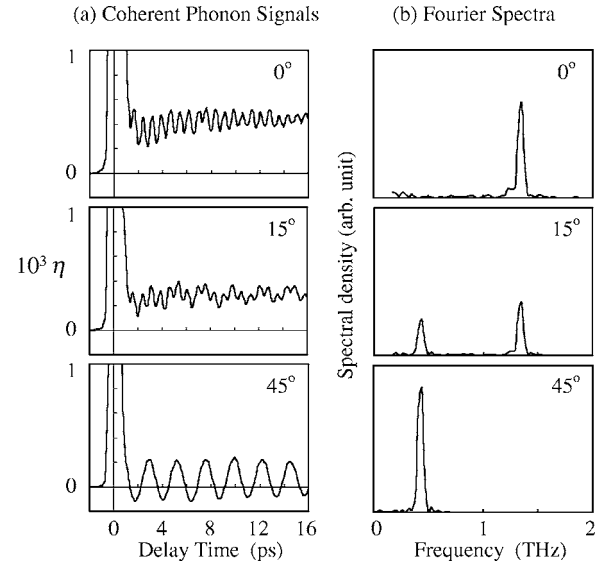
FIG. 2. (a) Coherent phonon signals at 6 K observed for 0^\circ , 15^\circ , and 45^\circ pumping, where the angle between the [100] axis of the crystal and the polarization direction of the pump pulse is changed. (b) Fourier transform of the coherent phonon signals in (a).
