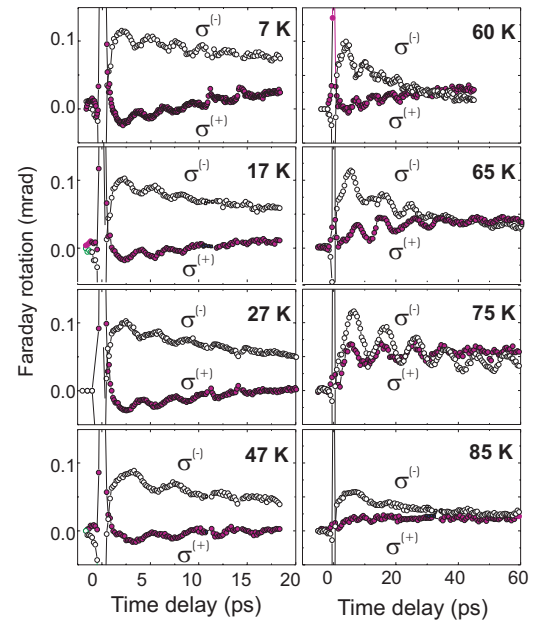
FIG. 2. (Color online) Magnetic excitations by circularly polarized pump pulses in \text{TmFeO}_3 probed by the magneto-optical Faraday effect.
