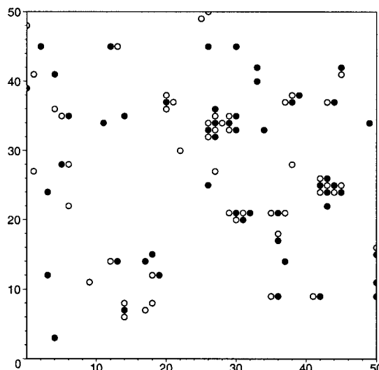
FIG. 2. “Defects only” view of Fig. 1. The full circles represent excess particles, while the empty circles are vacancies. The sites which are filled according to the regular “chessboard” pattern are not shown.
