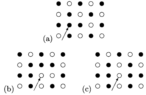
FIG. 11. Essential configurations for excess particle monomer: (a) excess particle monomer, (b,c) transient states. Centering is indicated by arrow.
