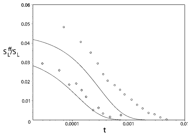
FIG. 13. Relative contribution of fluctuations due to flip-flop jumps for \phi=2.7 (top) and 3.0 (bottom), L=6 . Circles and diamonds are MC data, while full lines are theoretical calculations.
