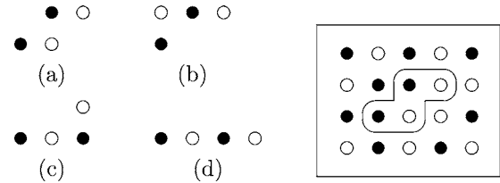
FIG. 6. Generation-recombination precursors. The structural defect (a) is also depicted in the box to show its position with respect to the sublattices.
