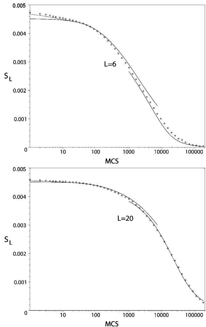
FIG. 14. Correlation function of fluctuations in probe area per site vs MC steps for \phi=2.70 , c=0.5 , L is indicated. 1 MCS corresponds to time [4(1+e^\phi)(1+e^{2\phi})]^{-1} . Circles are MC data. The solid line at short times is the correlation function of fluctuations due to random walk of monomers only given by Eq. (31). The dash line (merging with solid at 20 MCS) is the same quantity with flip-flop jumps accounted as well [Eq. (36)]. The solid line at long times is the correlation function of fluctuations from the diffusion and recombination of monomers from Ref. 5.
