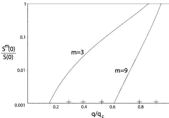
FIG. 8. Relative contribution of long-distance components of the correlation function to S(0) at exact half filling according to Eq. (9) depending on interaction strength q/q_c \equiv e^{\phi_c - \phi} . Parameters of MC simulations (see Sec. VII) are marked by crosses on the horizontal axis \phi = \{3.0, 2.7, 2.4, 2.0, 1.86\} (from left to right).
