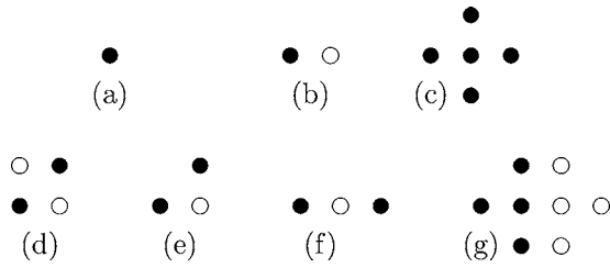
FIG. 4. All structural defects up to q^4 level: (a) excess particle, (b) flip-flop pair, (c) excess particle monomer, (d) flip-flop tetrad, (e,f) transient configurations during monomer jump, (g) isolated flip-flop pair. Only essential sites are shown, positions with respect to sublattices can be easily guessed. Configurations obtained by color inversion must be also included.
