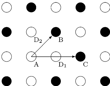
FIG. 10. Displacement of vacancy monomer.
