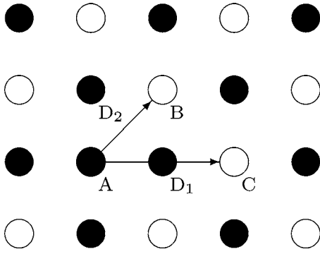
FIG. 9. Displacement of excess particle monomer.
