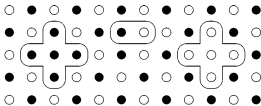
FIG. 5. Structural defects at q^3 level, from left to right: excess particle monomer, flip-flop pair, vacancy monomer. The sites defining each defect are encircled.
