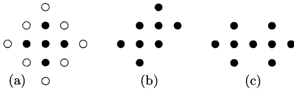
FIG. 7. (a) Isolated monomer, (b) side and (c) corner dimers of excess particle.
