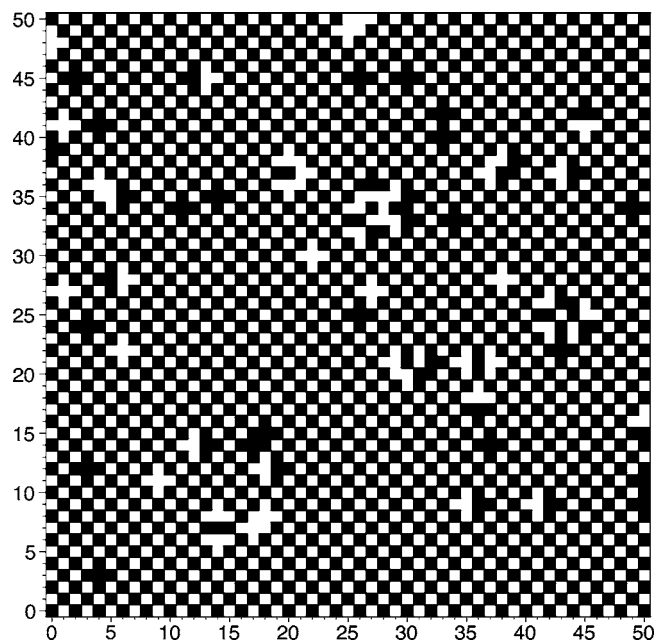
FIG. 1. A snapshot for \phi=2.0 and c=0.5 . A black square is an excess particle (occupied site), while a white square is a vacancy (empty site).
