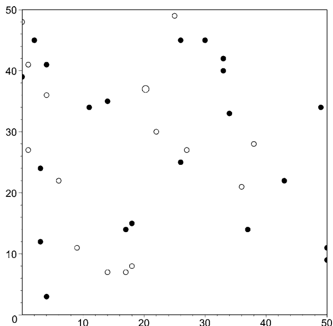
FIG. 3. Snapshot of the topological charges after the subtraction of the excess particle-vacancy pairs. The large circle in the upper middle of the picture is a dimer of vacancies.
