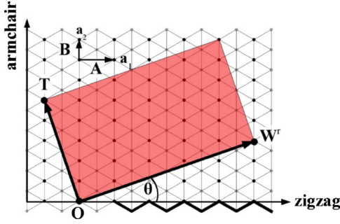
FIG. 14. (Color online) The geometrical construction of an ideal boron nanotube from a boron sheet: the red (gray) area is cut and rolled up such that \mathbf{W}^r will become the circumference of the nanotube. \mathbf{O} is the origin, \mathbf{W}^r is the wrapping vector, \mathbf{T} is the translational vector, \theta is the chiral angle measured with respect to the zigzag direction, \mathbf{a}_{1,2} are the primitive vectors of the underlying rectangular lattice, and A and B are the lattice constants (see text). The puckering of the boron sheet is indicated by black and gray atoms in the background. The zigzag and the armchair directions are perpendicular to each other. This figure corresponds to \mathbf{W}^r = (5, 3) and A/B = \sqrt{3} , which implies \mathbf{T} = (-1, 5) .
