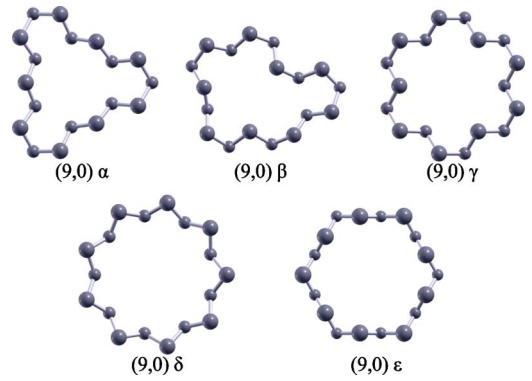
FIG. 7. (Color online) The cross sections of different isomers of a free standing (9,0) zigzag boron nanotube. The big spheres stand for the upper atoms and the small ones for the lower atoms (with respect to the direction of the tube axis). The \alpha and \gamma isomers are the free standing counterparts of the (9,0)C and (9,0)B tubes in Ref. 17, respectively.
