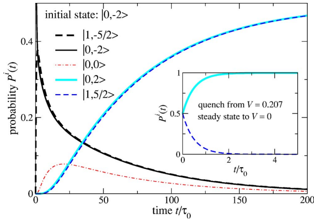
FIG. 4. (Color online) Probabilities of molecular states after initial preparation in state |0, -2\rangle as functions of time at the bias voltage V=0.207 V. The probabilities of states with extremal spin polarization and of the representative intermediate state |0, 0\rangle are shown. A magnetic field ( B=0.002 ) leads to spin relaxation towards larger spin values. The parameters are T=0.0002 (lower than before), K_2=0.04 and otherwise as in Fig. 2(a). Inset: Probabilities after the bias voltage is suddenly switched off in the steady state reached for V=0.207 V.
