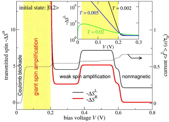
FIG. 3. (Color online) Total transmitted spin through the left and right leads for a magnetic molecule prepared in the n=0 maximum spin state |0, 2\rangle , as functions of bias voltage. The parameters are as in Fig. 2 with K_2=0.04 . The steady-state current is also shown. The inset shows the spin transmitted through the left lead on a logarithmic scale as a function of bias voltage for three different temperatures. 20
