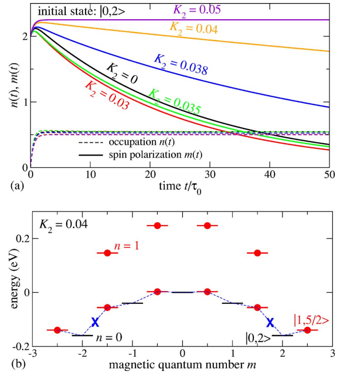
FIG. 2. (Color online) (a) Occupation n(t) and spin polarization m(t) for bias V=0.2 V, and T=0.002 , S=2 , \epsilon=0.12 , U=1 , J=0.1 , and B=0 for various anisotropies K_2 . In this and the following figures we absorb the gate voltage into \epsilon . The molecule is in state |0, 2\rangle at time t=0 . (b) Molecular energy levels for states with n=0 (black bars) and n=1 (red/gray bars with circles) for the parameters from (a) and K_2=0.04 . Active transitions are denoted by dashed lines. The crosses denote the transitions that next become thermally suppressed for larger K_2 or smaller bias V .
