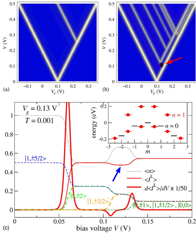
FIG. 1. (Color online) dI/dV as a function of gate voltage V_g and bias voltage V . Yellow (bright) colors denote positive values of the differential conductance, dark red (dark gray) colors denote negative values. In (a) results for an isotropic molecule are shown, the parameters are T=0.002 , S=2 , \epsilon=0.2 , U=1 , J=0.1 , K_2=B=0 . Energies are here and in the following given in electron volts. Coulomb blockade is found to the left and right of the V-shaped region, whereas within this region a nonzero steady-state current is flowing. The satellite line results from the exchange splitting of energy levels for n=1 . In (b) an anisotropy of K_2=0.04 has been assumed, leading to a complex splitting of the dI/dV peaks. We find one peak with NDC (arrow). (c) Occupation, steady-state current in units of e/\tau_0 , dI/dV in units of e/\tau_0 per volt, and probabilities of various states (dashed) for a cut through the NDC region in (b) at the lower temperature T=0.001 . The arrow indicates the plateau with reduced current. Inset: Molecular energy levels of states with n=0 (black bars) and n=1 (red/gray bars with circles) and magnetic quantum numbers m .
