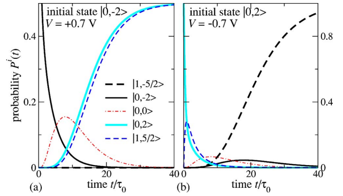
FIG. 5. (Color online) Probabilities of molecular states after initial preparation in state (a) |0, -2\rangle and (b) |0, 2\rangle as functions of time at the bias voltage (a) V=+0.7 V and (b) -0.7 V. The right lead is ferromagnetic with a ratio of densities of states of D_{\downarrow}^R/D_{\uparrow}^R=0.001 . There is no applied magnetic field. The other parameters are as in Fig. 4 except for the much higher temperature T=0.02 .
