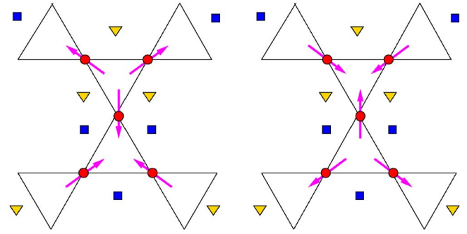
FIG. 8. (Color online) Spin structure of FeJ. The squares (blue) are sites in the Kagomé plane at z=c/3 , the triangles (yellow) are sites in the plane at z=-c/3 , and the circles (red) are sites in the plane at z=0 . The two symmetry related choices for spin orientations in the ordered phase are shown in the two panels.
