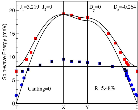
FIG. 13. (Color online) Spin-wave spectrum from a simple two-parameter J_1 - D_z model. In these and succeeding figures the values of the parameters of the fit are given in meV.
