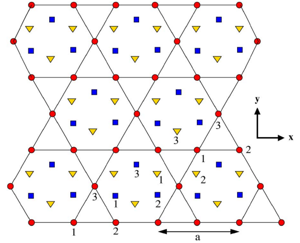
FIG. 3. (Color online) Kagomé planes. The solid circles are x - y planes at z=0 , the solid squares are x - y planes at z=c/3 , and the solid triangles are x - y planes at z=2c/3 . The positive z axis is out of the plane. Representative sublattice numbers \tau are given.
