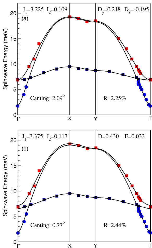
FIG. 16. (Color online) Spin-wave spectrum from isotropic NN and NNN interactions J_1 and J_2 and (a) DM vector (0, D_y, D_z) and (b) single-ion anisotropy terms D and E .
