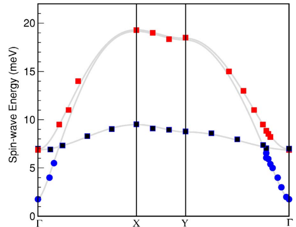
FIG. 12. (Color online) Experimental spin-wave spectrum in FeJ obtained from inelastic neutron scattering measurements (Ref. 22). The gray lines represent the best fit which is discussed in the text in detail.
