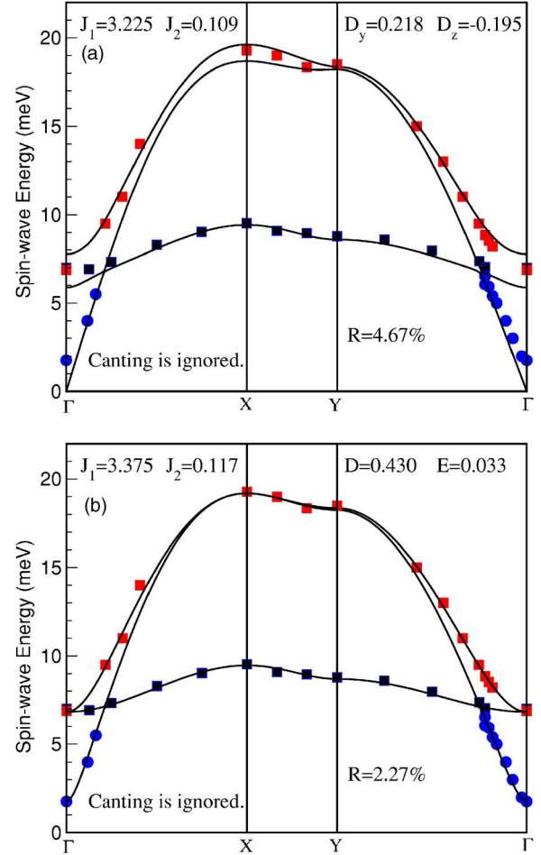
FIG. 17. (Color online) Spin-wave spectrum for the DM (a) and CF (b) models when the spin canting is ignored. We used the same parameters as in Fig. 16 to emphasize the effect of spin canting on the spectrum.
