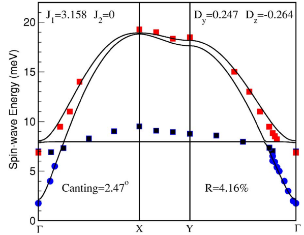
FIG. 14. (Color online) Spin-wave spectrum from a simple three-parameter J_1 - D_y - D_z model.
