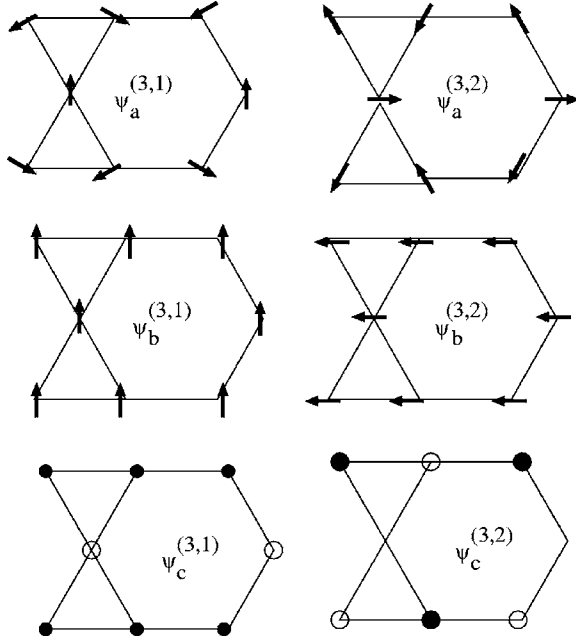
FIG. 6. Spin configurations which transform according to two-dimensional irrep \Gamma_3^+ . In the left (right) column we give the wave functions which transform according to the first (second) row of the matrices of the irrep. Arrows represent spins of unit length. Solid (open) circles indicate spins pointing perpendicularly into (out of) the Kagomé plane. For \Psi_c^{(3,1)} the magnitudes of the inward spins are both equal to half that of the outward spin which is set to be \sqrt{2} . For \Psi_c^{(3,2)} the nonzero magnitudes of the spins are both \sqrt{3}/2 .
