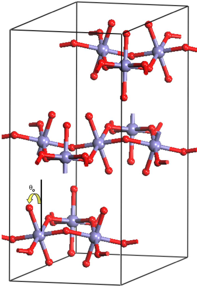
FIG. 2. (Color online) Conventional unit cell of FeJ. For clarity only Fe, large spheres (blue), and the octahedral oxygen atoms, small spheres (red), are shown. The tilting angle \theta_0 of the \text{FeO}_6 octahedra is also shown.
