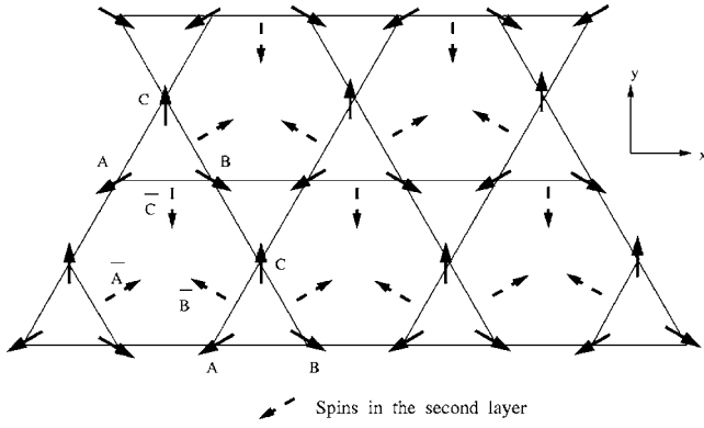
FIG. 7. Spin structure of FeJ as determined in Refs. 14, 16, and 21.
