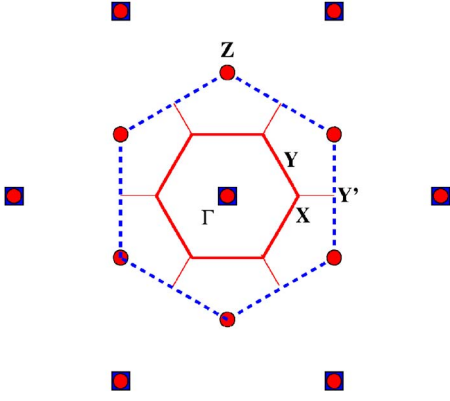
FIG. 4. (Color online) Reciprocal lattices for the FeJ system (blue squares) and for the two-dimensional hexagonal lattice (red circles). The first Brillouin zone for the two-dimensional hexagonal system is indicated by heavy solid lines in red and that (in the z=0 plane) for the FeJ system by heavy dashed lines in blue. The light solid lines in red mark the boundaries of neighboring hexagonal zones. The FeJ Brillouin zone is 3 times as large as the hexagonal zone.
