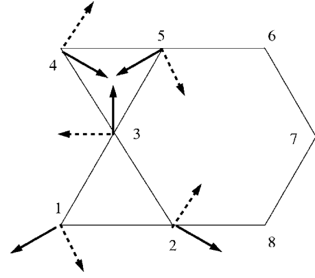
FIG. 10. Local axes of various sites. The local z axis (indicated by the solid lines with arrows) is along the projection of the direction of the local magnetization onto the Kagomé plane. The local y axis is perpendicularly out of the Kagomé plane. The local x axis is in the Kagomé plane and is indicated by the dashed lines with arrows.
