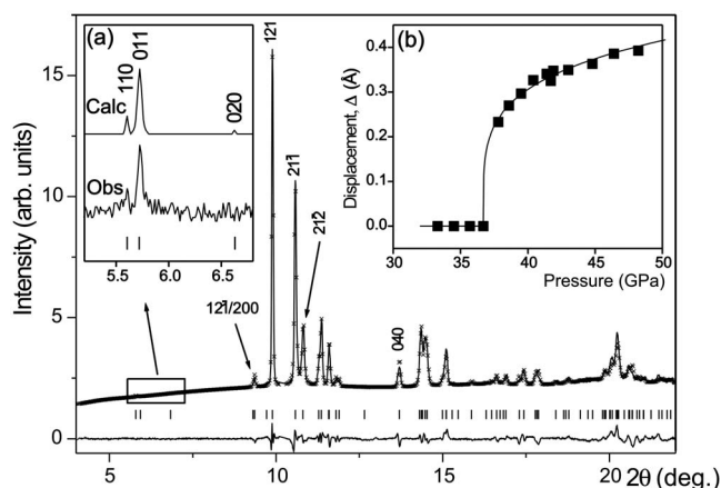
FIG. 4. Constrained Rietveld refinement of Sr-IV at 41.7(3) GPa with model (iii) (see text). The tick marks and difference profile are shown as in Fig. 3. Inset (a): ESRF data for the range marked, compared with the calculated profile for constrained model (iii). Note that this inset is not an enlargement of the main profile fit, which uses the same SRS data as Fig. 3. Inset (b): pressure dependence of the helical displacement \Delta as obtained from the constrained refinements (see text). The estimated errors are approximately the same as the size of the symbols. The line through the points is a guide to the eye.
