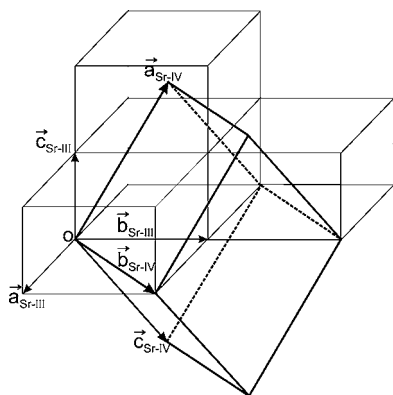
FIG. 2. Relationship between the unit cells of the Sr-III phase (light lines) and the superstructure Sr-IV phase (heavy lines).
