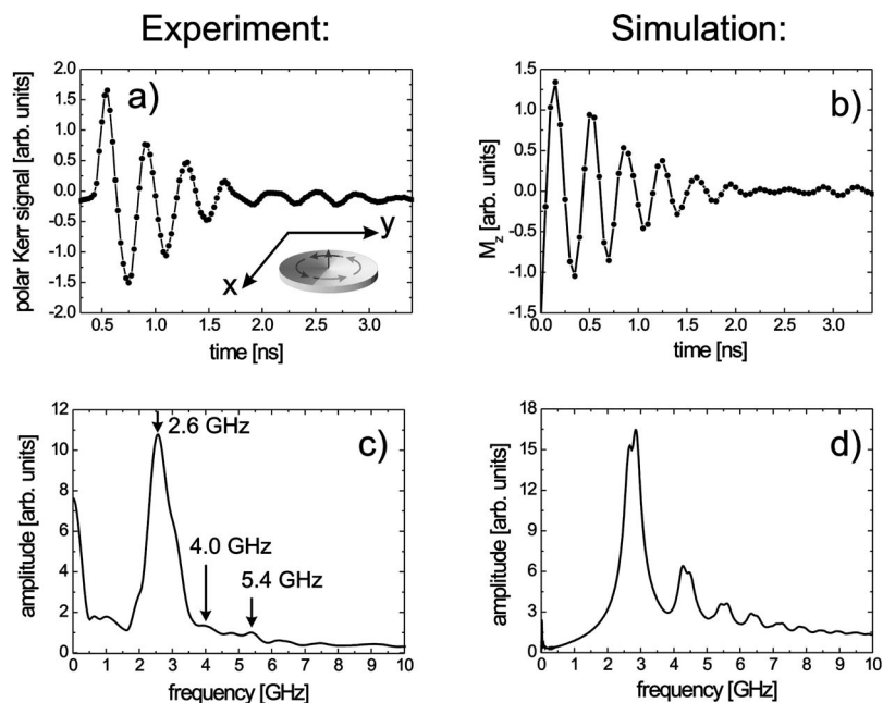
FIG. 3. The z component of the magnetization \mathbf{M} as a function of time obtained from time-resolved magneto-optic Kerr microscopy (a) and from micromagnetic simulation (b) averaged over one half of the disk [see inset in (a)]. The corresponding Fourier transform of the experimental and the simulated data is shown in (c) and (d), respectively.
