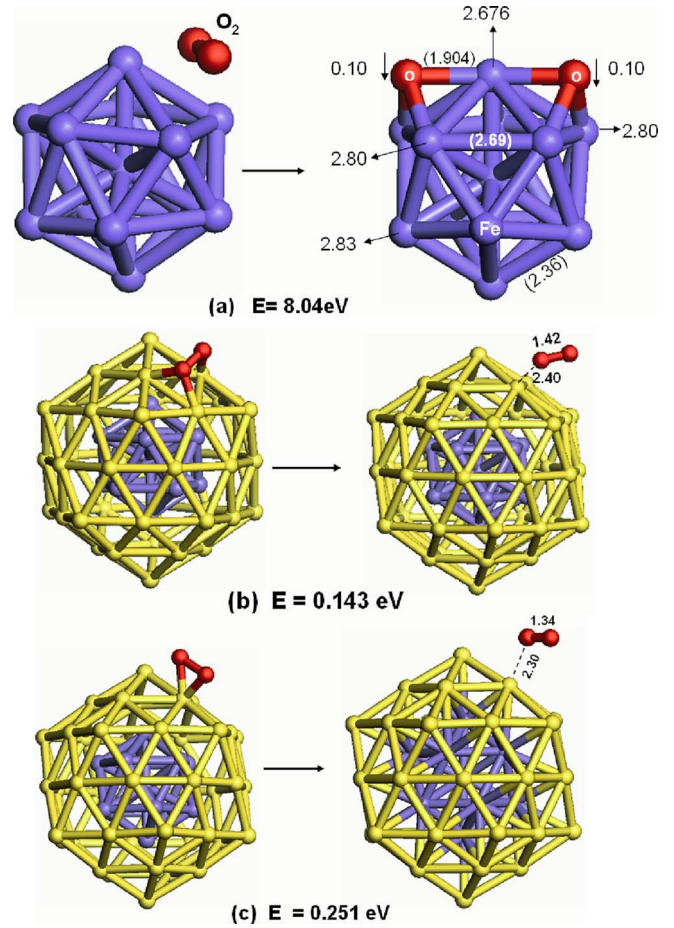
FIG. 7. (Color online) Initial and optimized geometries for Fe 13 -O 2 and Fe 13 @Au 42 -O 2 . The bond length (in Å, the numbers in parentheses) and moment (in μ B ) are given for Fe 13 -O 2 . The bond length of O 2 and the distance between O 2 and Au shell are shown in (b) and (c).
