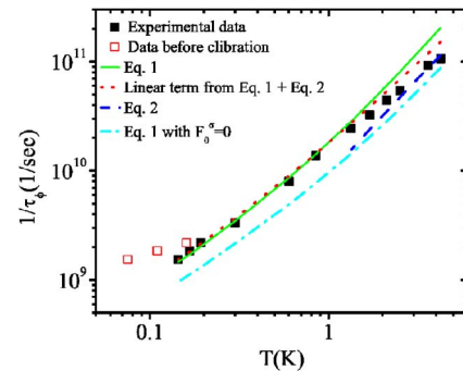
FIG. 3. (Color online) The temperature dependence of the dephasing rate \tau_\phi^{-1} extracted from the weak-localization measurements (black squares). The green solid line is the theoretical value from Eq. (1). The blue dashed line is the theoretical value from Eq. (2). The red dotted line is the theoretical value from the combination of the linear term in Eq. (1) and Eq. (2). The cyan dashed-dotted line represents the data for F_0^\sigma = 0 . The red empty squares represent the data for low temperatures without temperature calibration.
