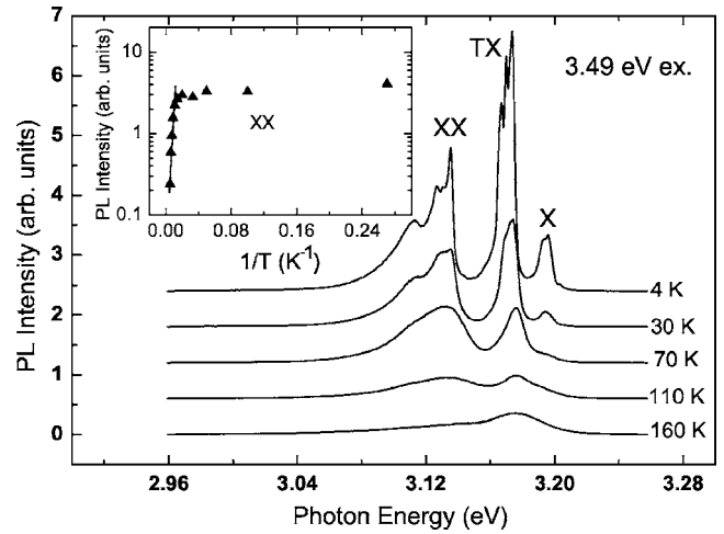
FIG. 3. PL spectra at different temperatures under excitation with 3.49 eV photons. The inset shows the temperature dependence of the XX intensity. A straight line represents thermal activation energy of 36 meV.
