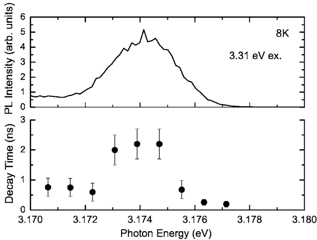
FIG. 2. The PL intensity and decay time as a function of the photon energy around the TX lines at 8 K are shown in the upper and lower panels, respectively. The excitation photon energy is 3.31 eV, and the spectral resolution is 1 meV.
