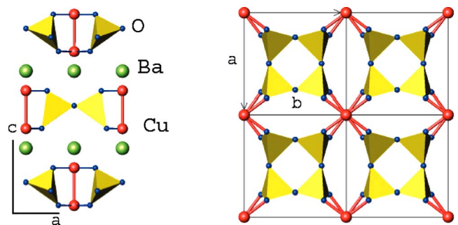
FIG. 1. (Color online) Schematic views of the room-temperature crystal structure of \text{BaCuSi}_2\text{O}_6 , composed of \text{SiO}_4 tetrahedra (Si atoms are located in tetrahedron centers), \text{CuO}_4 distorted squares, and Ba atoms. The \text{Cu}^{2+} ions in the \text{Cu}_2\text{Si}_4\text{O}_{12} layers form a quasi-two-dimensional system of weakly interacting dimers.
