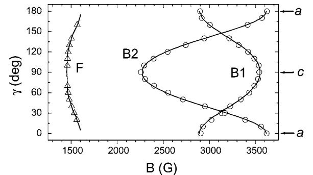
FIG. 4. Angular dependence of the EPR spectrum in \text{BaCuSi}_2\text{O}_6 in the ac plane, taken at a temperature of 6 K; \gamma is the angle between the direction of the applied field and the a axis. Triangles and circles correspond to experimental data, while lines correspond to stimulation results.
