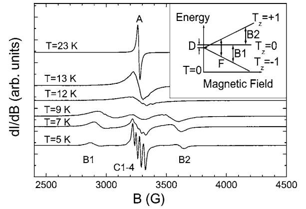
FIG. 3. The evolution of the low-temperature EPR spectra of \text{BaCuSi}_2\text{O}_6 ; the magnetic field is applied along the a axis. Note that points at lower temperatures are taken with an increased amplification rate. The lines A, B1 and B2 correspond to spin-triplet excitons. The hyperfine structure C1-4 is related to interactions within unpaired doublet \text{Cu}^{2+} sites, caused by defects. The line F (Fig. 4) is outside the shown field range. The inset shows a schematic view of the energy-level diagram for dimerized S=\frac{1}{2} systems in the tetragonal configuration.
