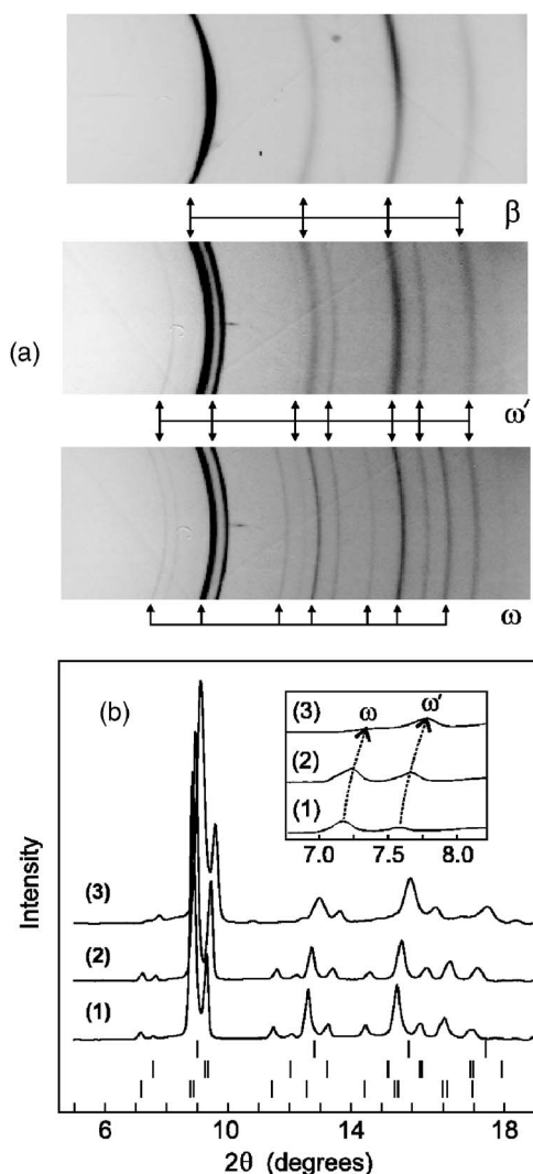
FIG. 2. Selected diffraction patterns of TiZr during a quasi-isothermal compression cycle at high temperature. (a) Debye-Scherrer diffraction rings of TiZr alloy as recorded on a CCD detector. The positions of diffraction rings assigned to \beta , \omega' , and \omega structures marked by arrows. (b) Integrated patterns collected at (1) 8.8 GPa, 815 K; (2) 18 GPa, 815 K; (3) 24.8 GPa, 745 K. The tick marks in (b) indicate the calculated peak positions for (from bottom to top) \omega , \omega' , and \beta structures. The inset shows the evolution of the (001) peaks from the \omega and \omega' structures in the angular range devoid of \beta -structure reflections.
