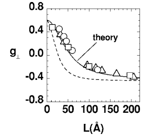
FIG. 10. g_{\perp} factor as a function of the QW width in GaAs-Ga 0.65 Al 0.35 As QWs. Theoretical results (full curve) are shown for B=4 T and for the orbit-center position at the center of the well (the dashed curve corresponds to theoretical results obtained by using a_1=a_2=\dots=a_6=0 ). Squares, circles, and triangles are the experimental data from Hannak et al. (Ref. 16), Le Jeune et al. (Ref. 17), and Malinowski et al. (Ref. 18), respectively.
