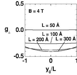
FIG. 8. g_{\perp} factor as a function of the orbit-center position in GaAs-Ga 0.65 Al 0.35 As QWs. Results are shown for various values of the width and for B=4 T.
